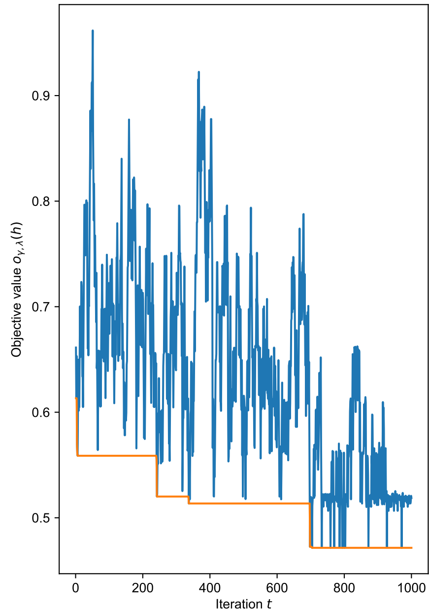
\gamma = 0.75, \lambda = 0.05
