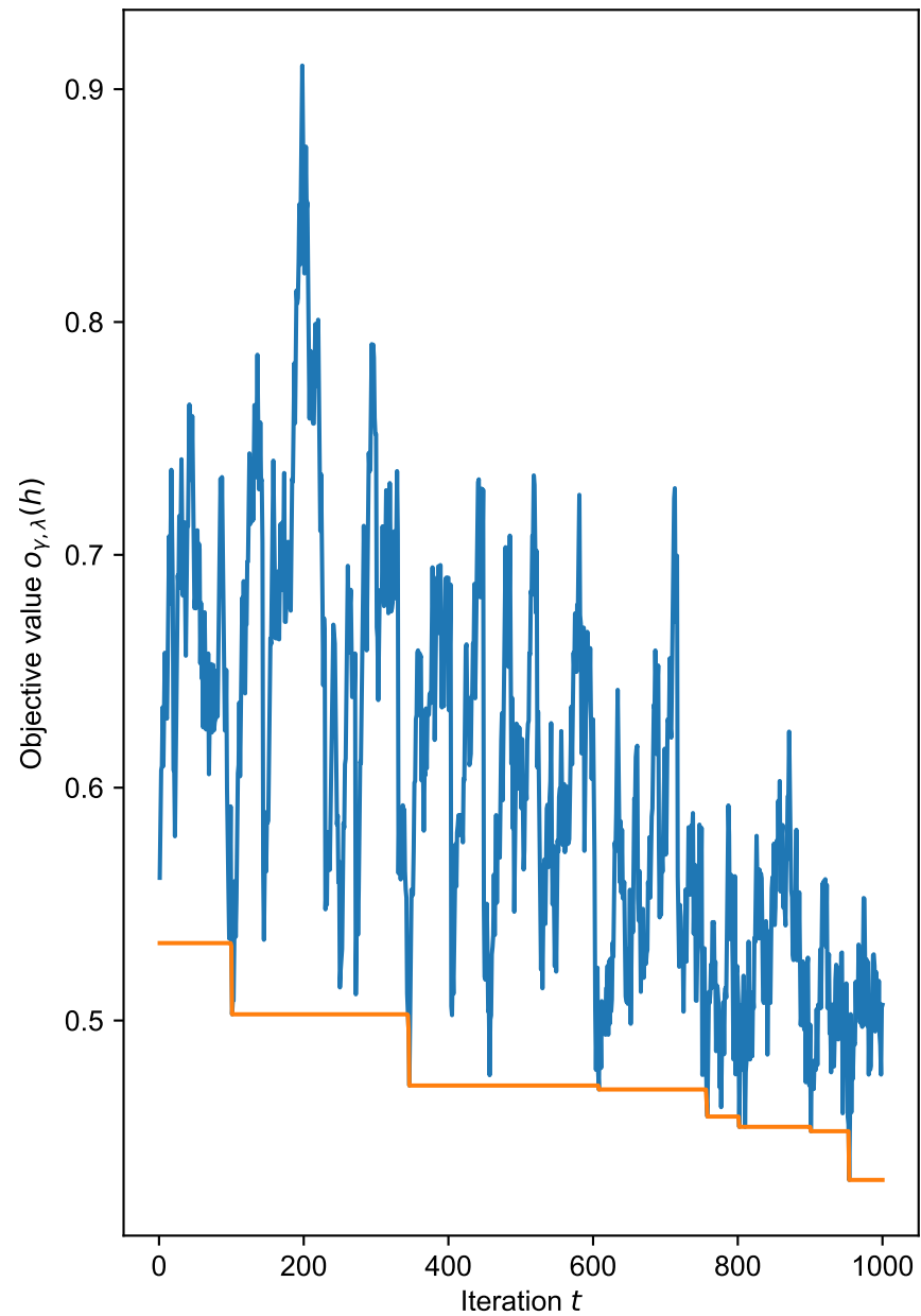
\gamma = 0.75, \lambda = 0.03
