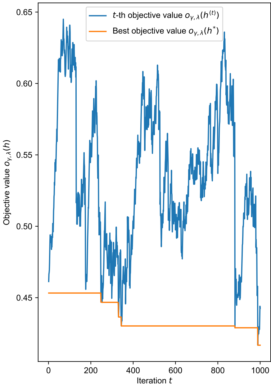
\gamma = 0.75, \lambda = 0.01
