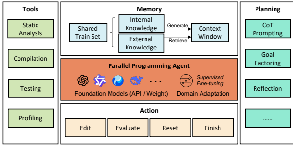
Figure 1. Architecture of Parallel Code Generation.
