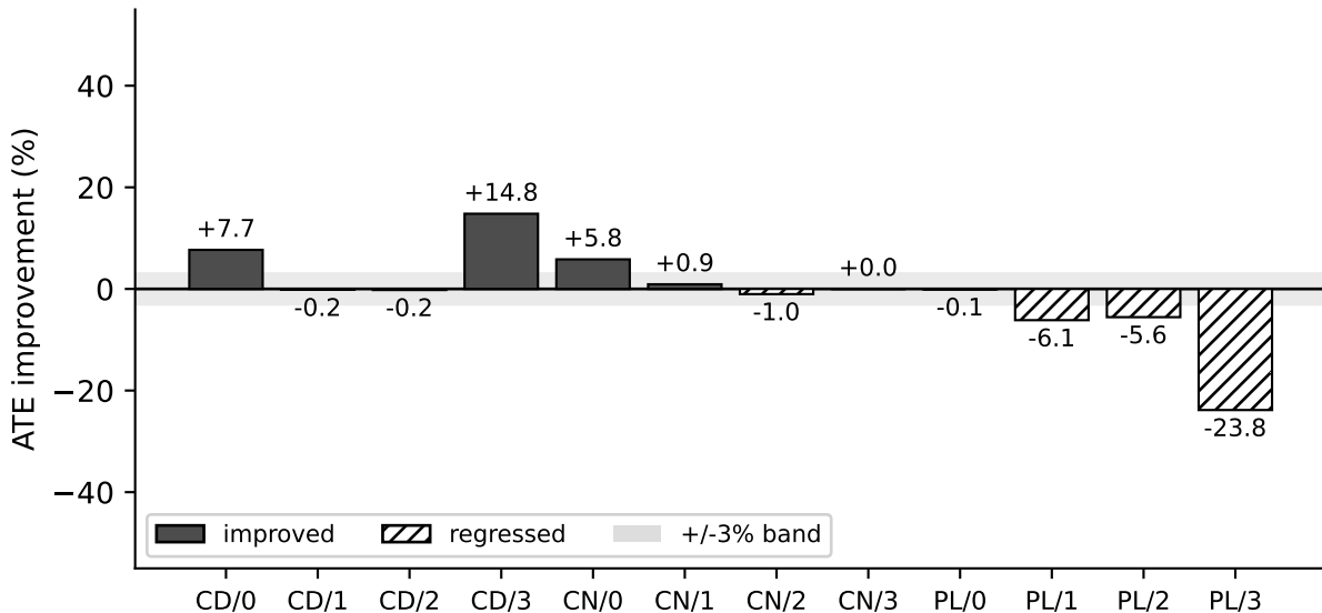
VIODE ATE improvement: GeoDF-Adaptive vs baseline [N=5 (measured)]
