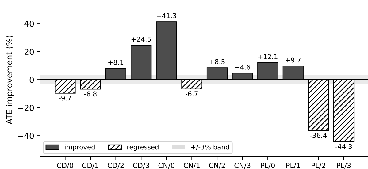
VIODE N=5 ATE improvement: GeoDF-Adaptive vs baseline
