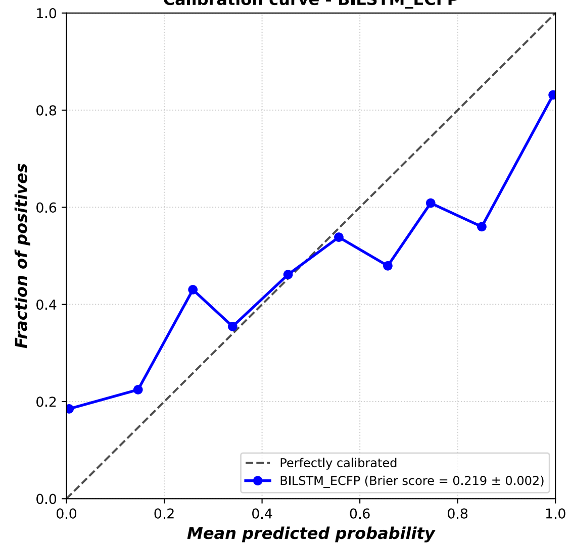
Calibration curve - BILSTM_ECFP
