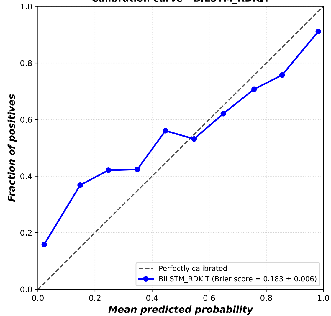
Calibration curve - BILSTM_RDKIT
