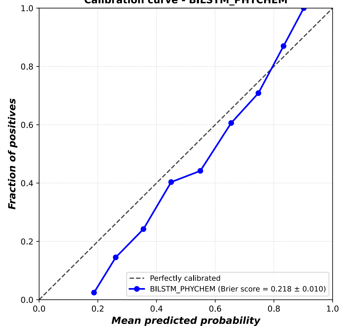
Calibration curve - BILSTM_PHYCHEM
