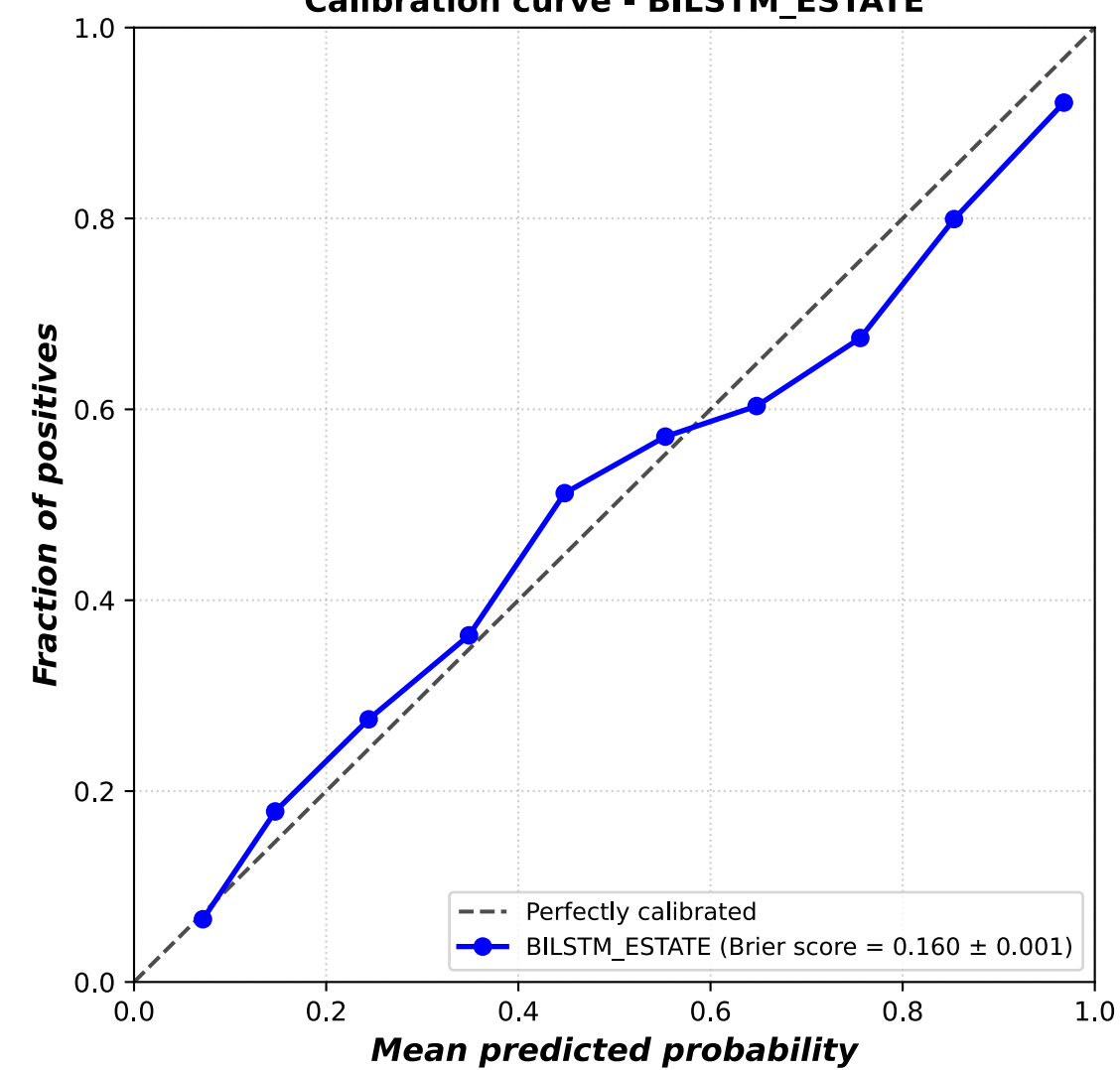
Calibration curve - BILSTM_ESTATE
