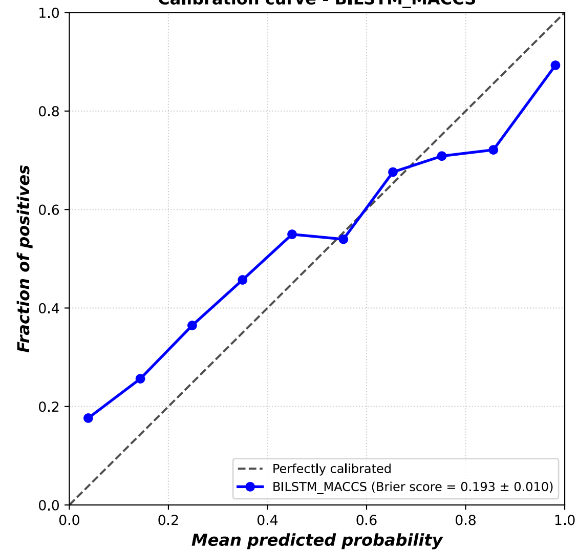
Calibration curve - BILSTM_MACCS
