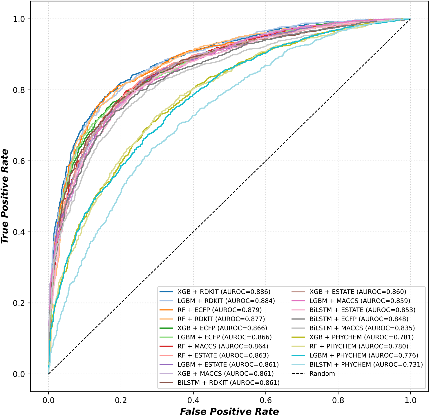
A AUROC comparison across 20 models
