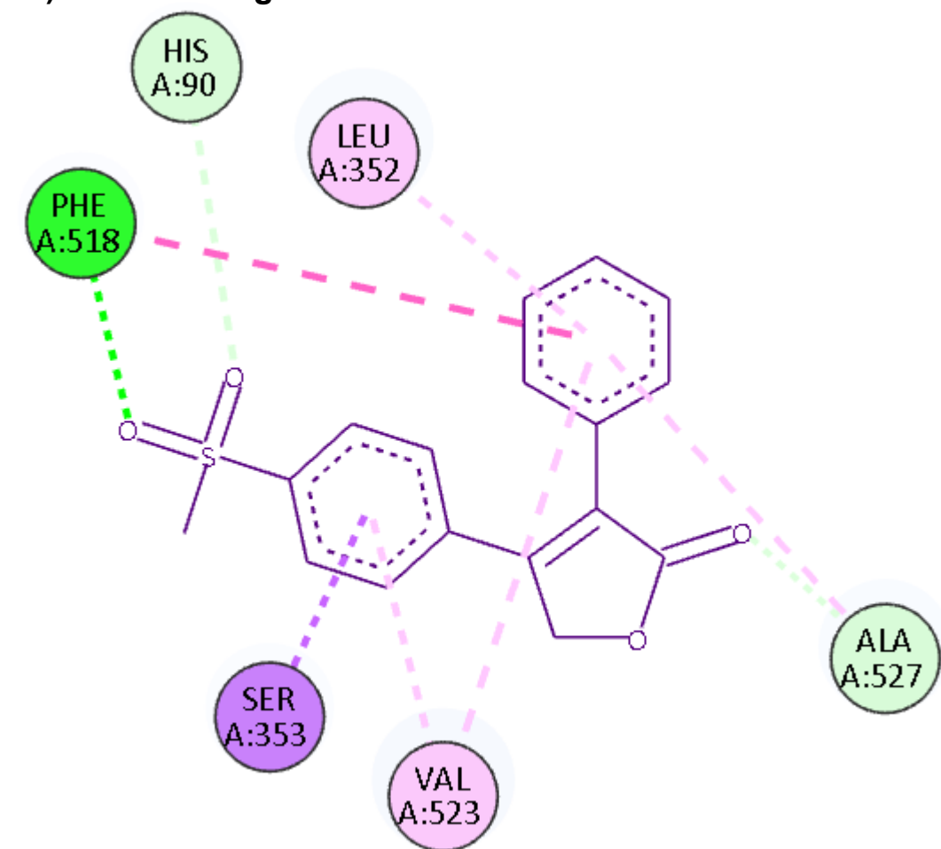
A) Reference ligand RCX
