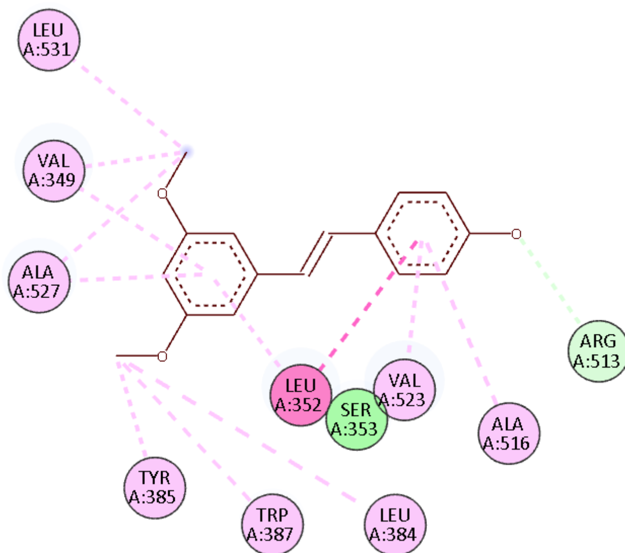
C) Ligand 20: 4-(2-(3,5-dimethoxyphenyl)ethenyl)phenol
