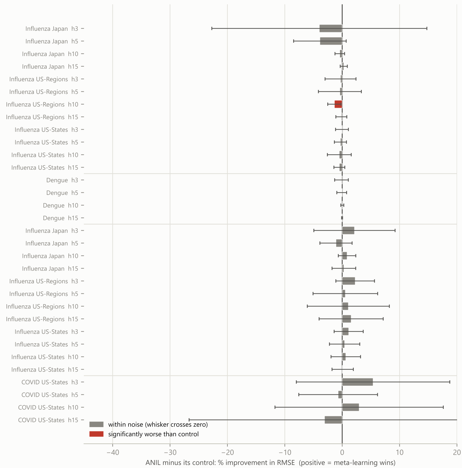
F2 Meta-learning against its own seed-matched control, 32 cells across 4 folds. RMSE, positive means ANIL beats the control; whiskers are the 95% t-interval.
