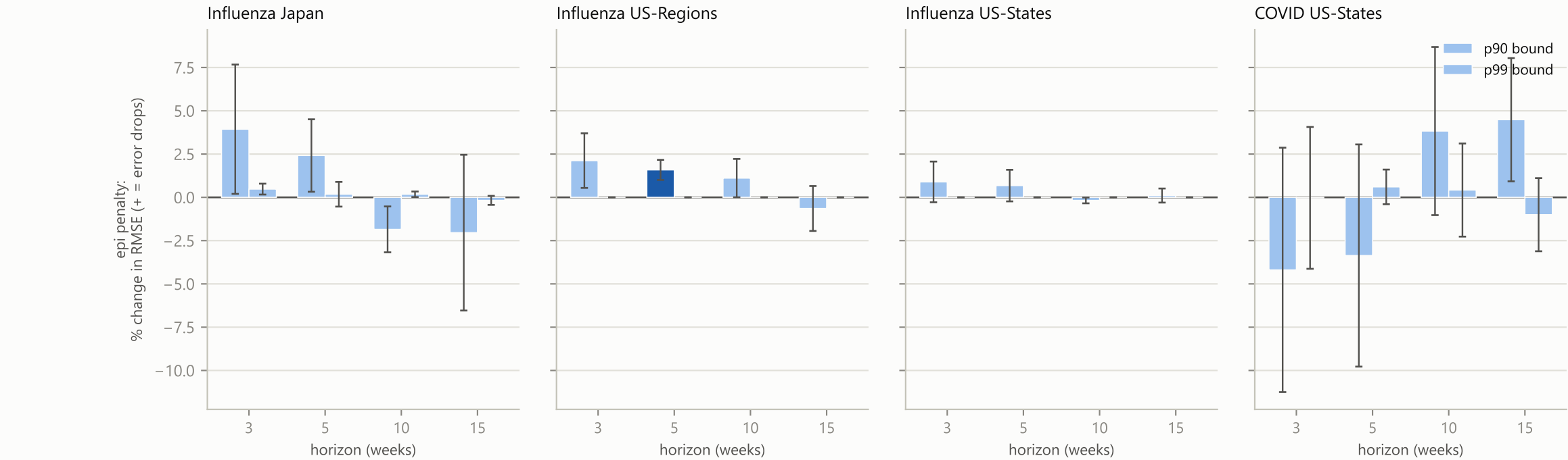
F3 Epidemiology-informed penalty. RMSE, lower is better; bars show the change from adding the penalty.
