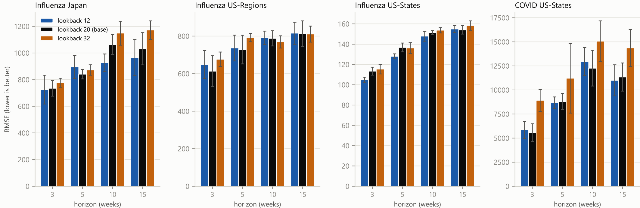
F4 Lookback window sensitivity. RMSE, lower is better; the base model uses lookback 20 (black).
