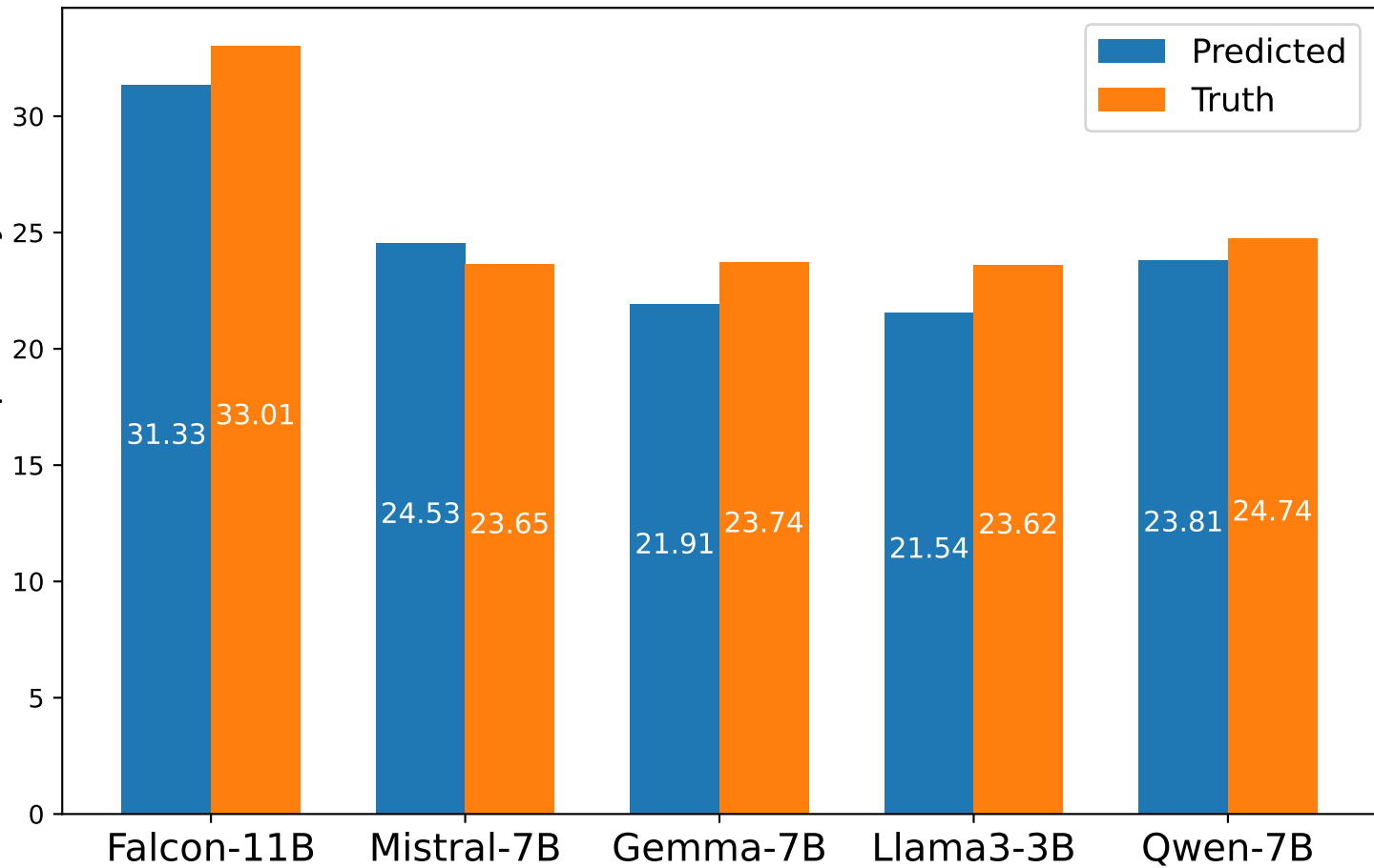
vLLM's Startup Latency (s)
