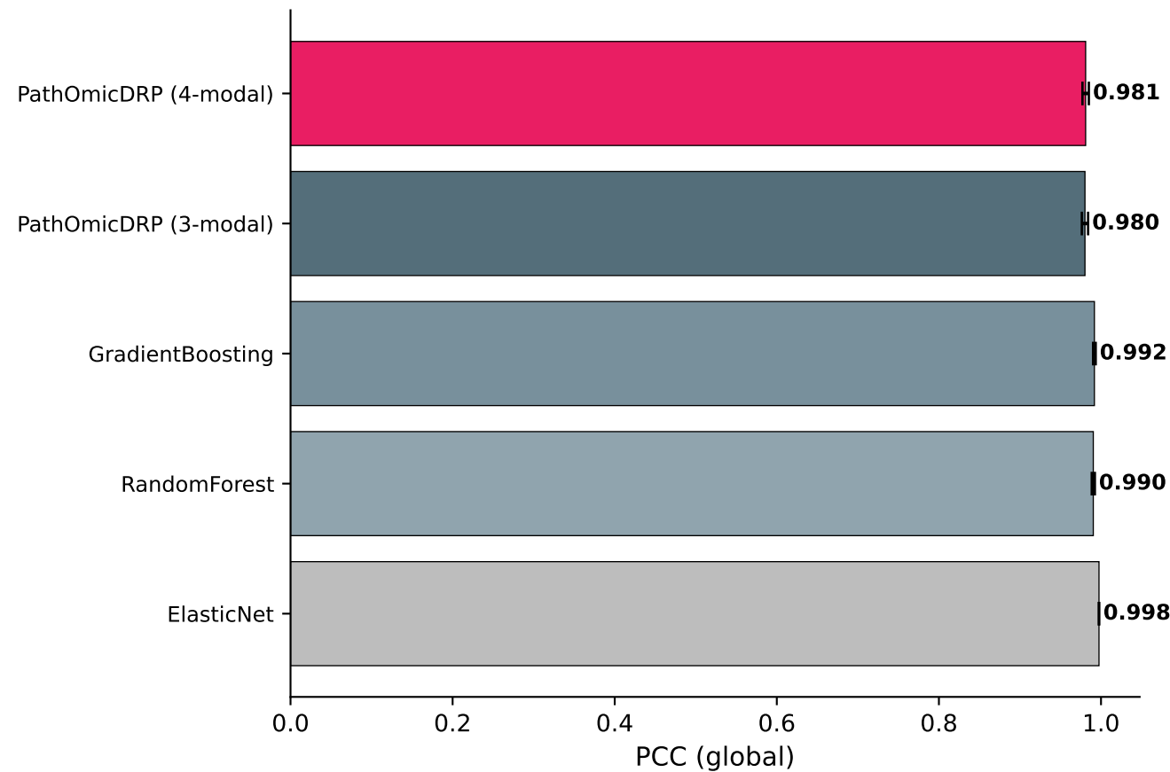
A Global Prediction Performance
