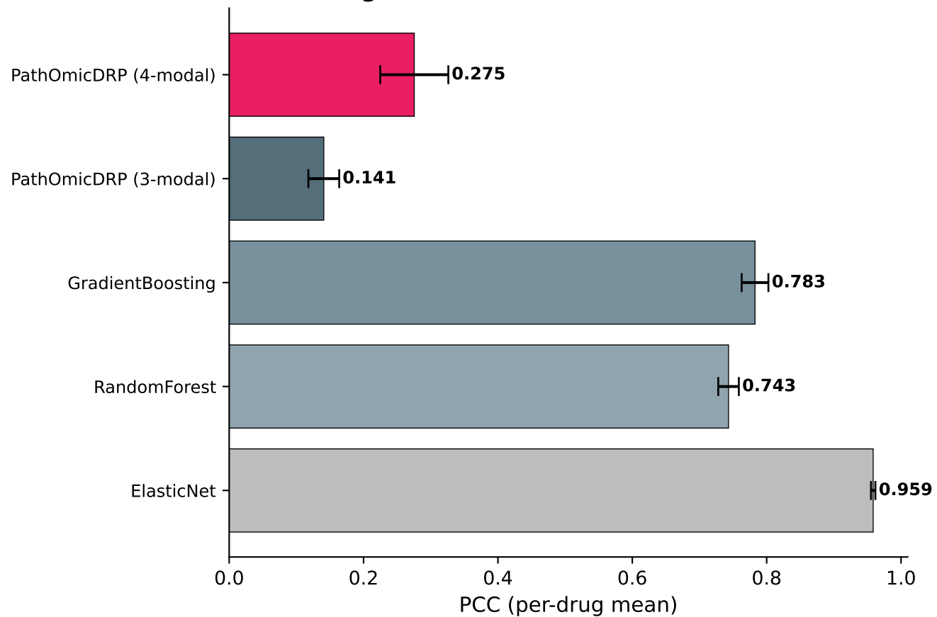
B Per-Drug Prediction Performance
