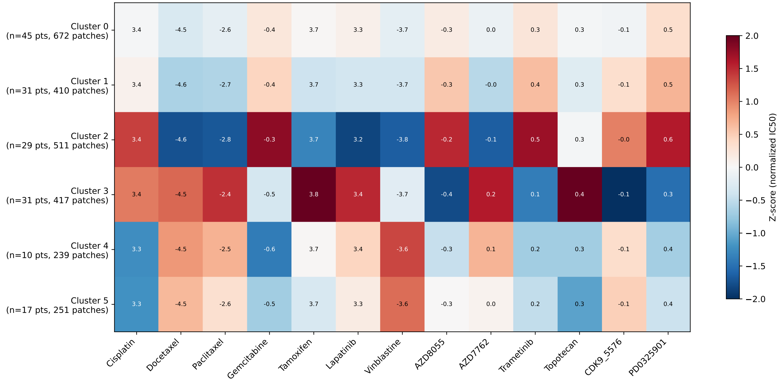
Tissue Phenotype Clusters: Drug Sensitivity Profiles (Z-scored predicted IC50, lower = more sensitive)
