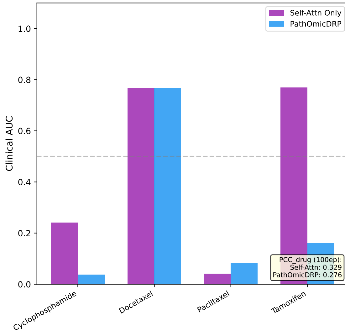
B. Cross-Attn vs Self-Attn Clinical AUC
