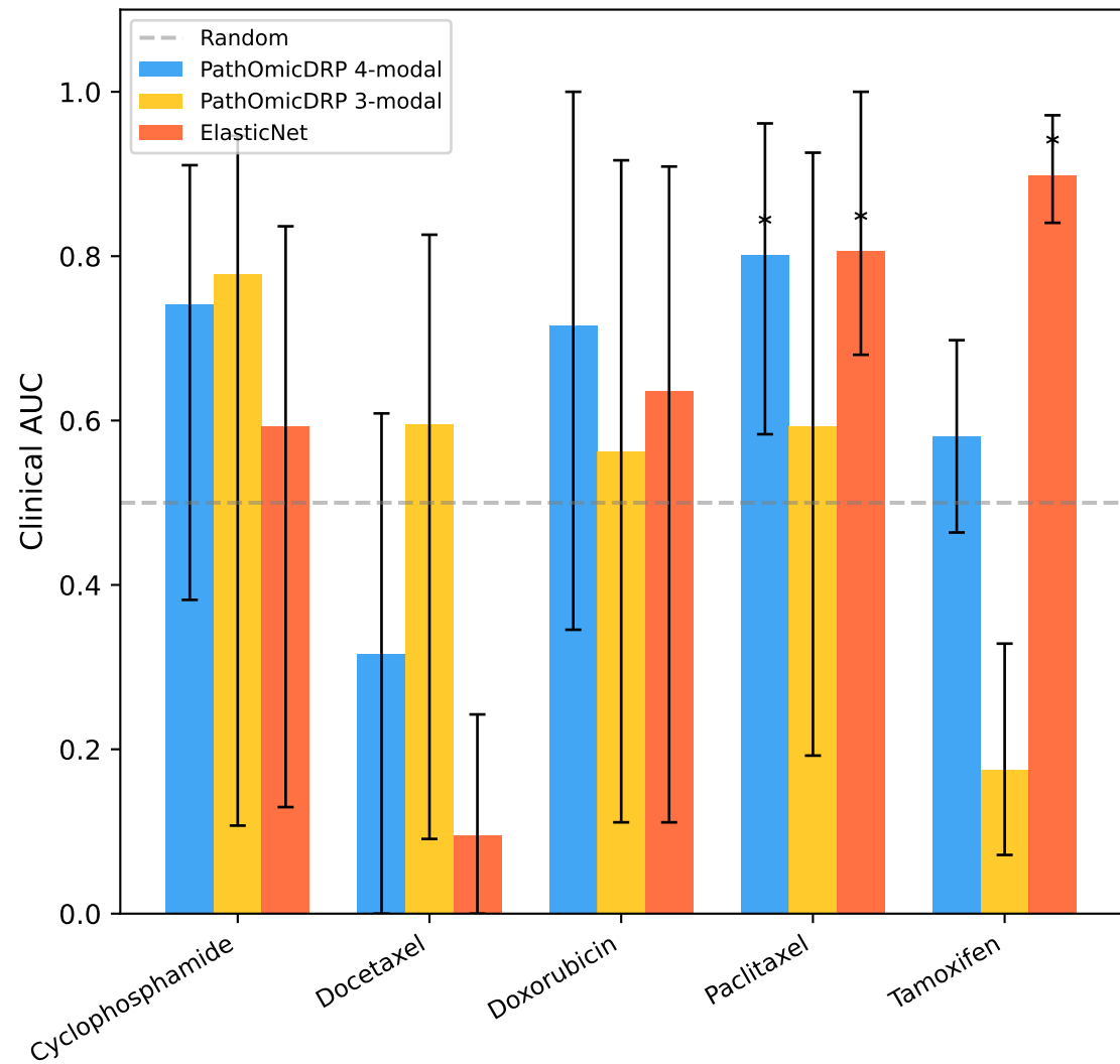
A. Clinical Outcome Prediction
