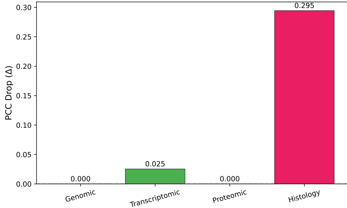
A. Modality Importance (PCC drop when ablated)
