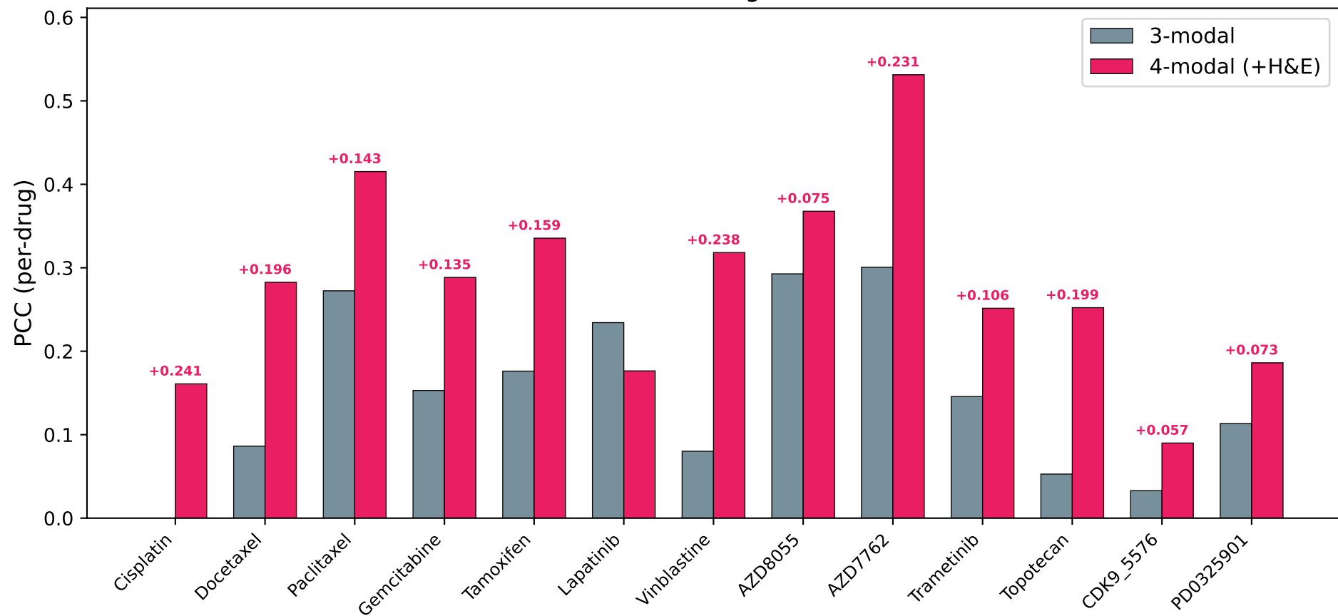
C. 3-Modal vs 4-Modal Per-Drug Prediction Performance
