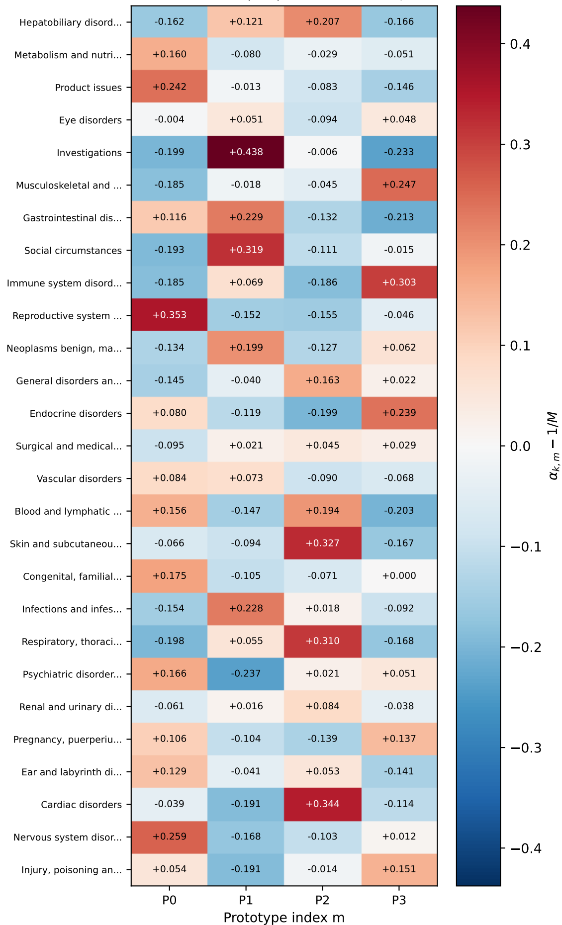
(b) \alpha - 1/M — max |dev| = 0.4377 (task-specific)
