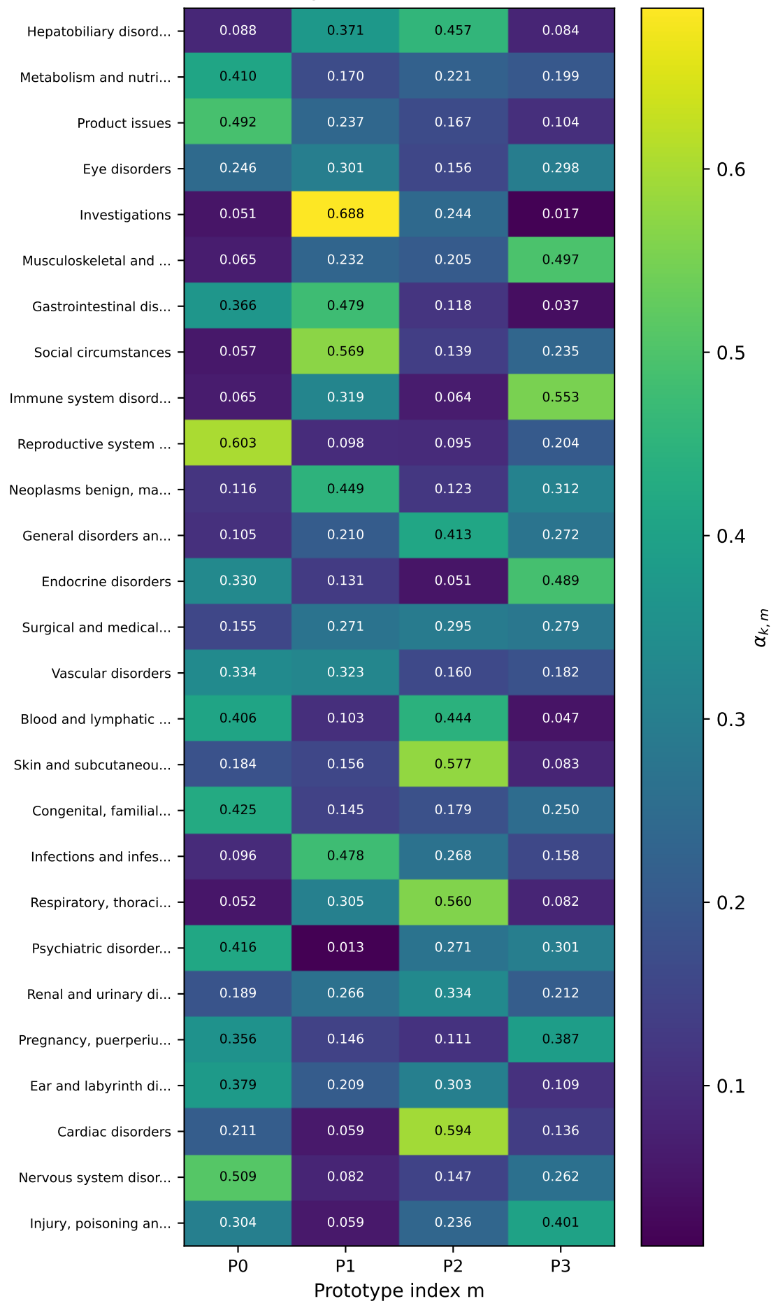
(a) raw \alpha — range [0.013, 0.688] uniform = 0.250
