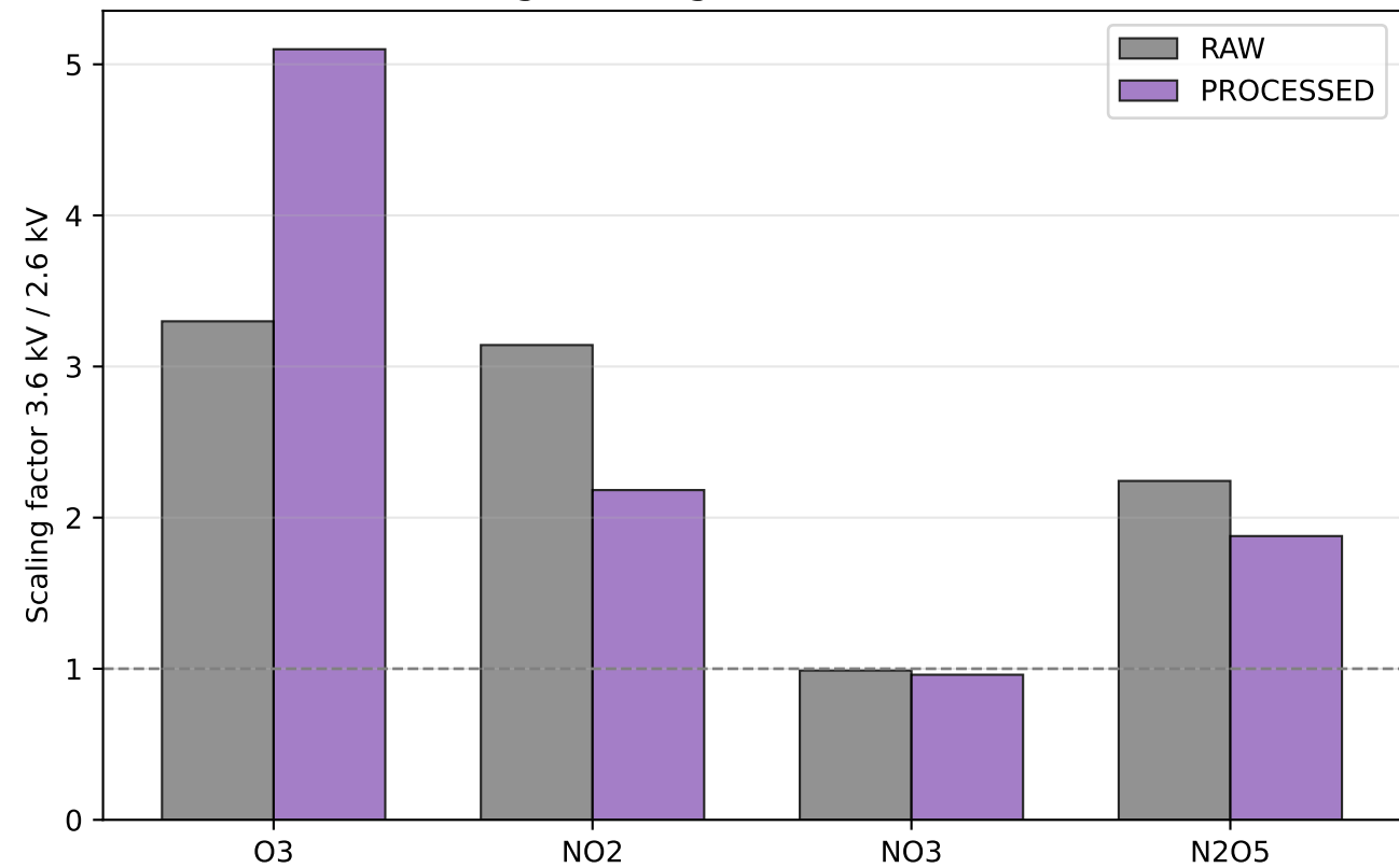
(b) Voltage scaling — RAW vs PROCESSED
