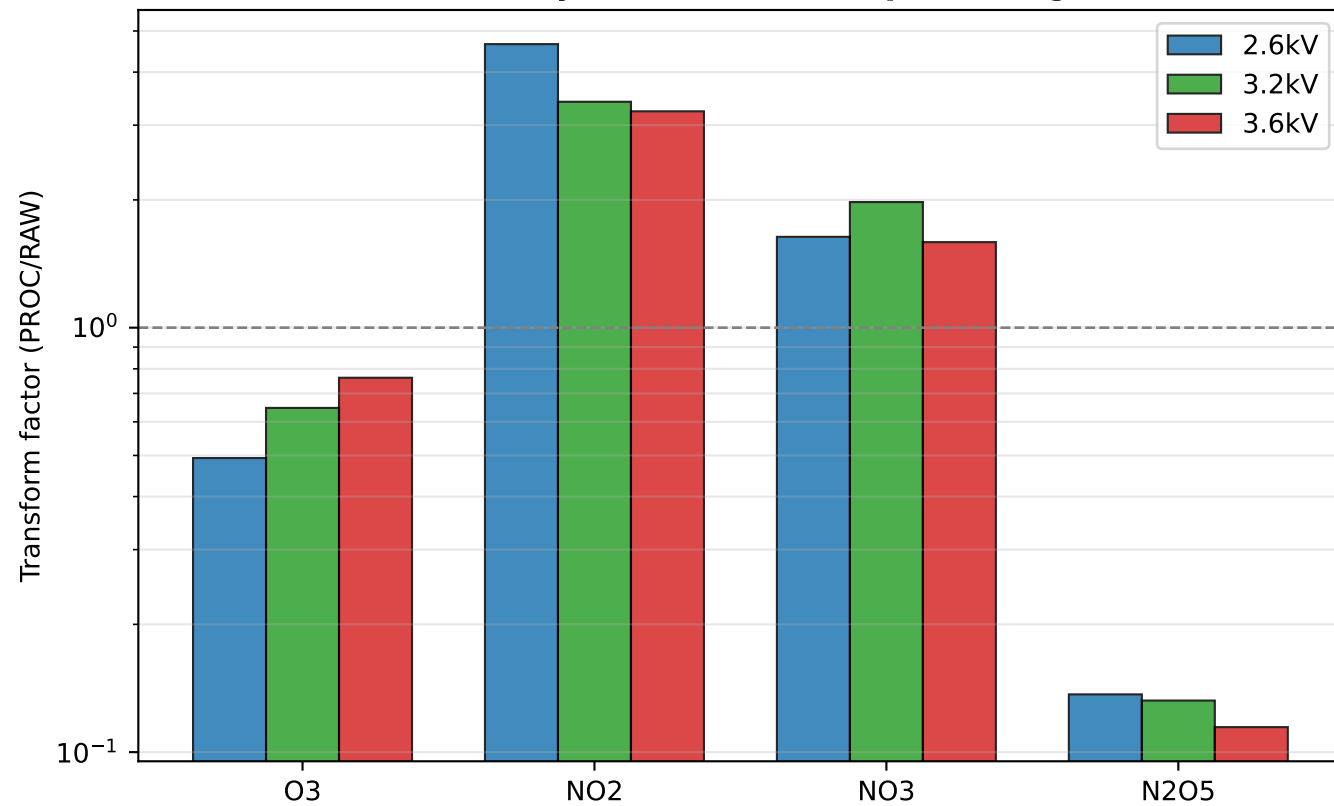
(a) Steady-state transform per voltage
