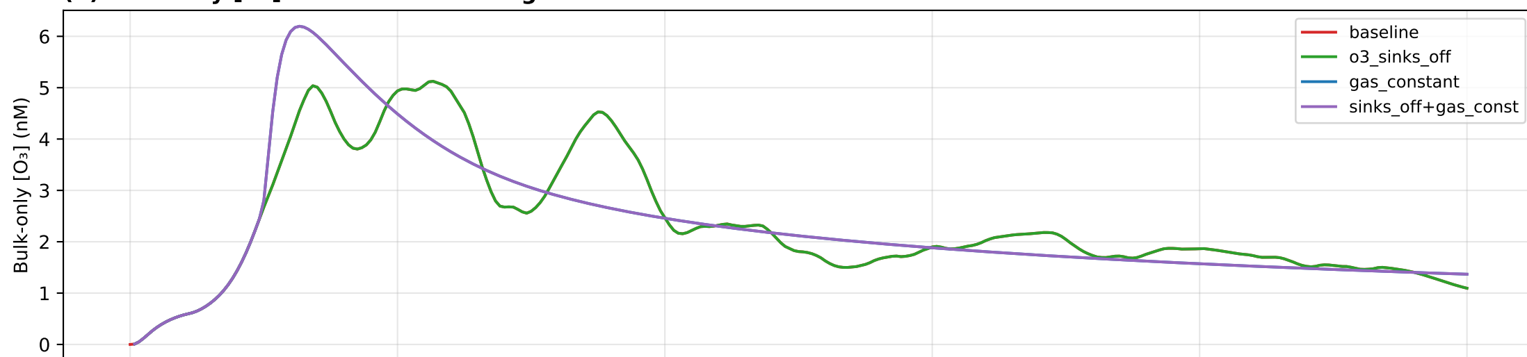
(b) Bulk-only [O 3 ] — z>0.1mm vol-avg
