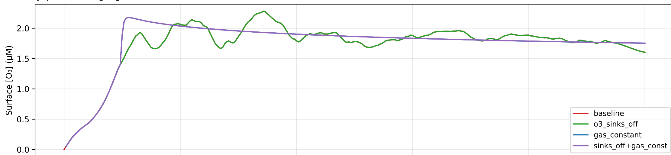
(a) Surface [O 3 ]
