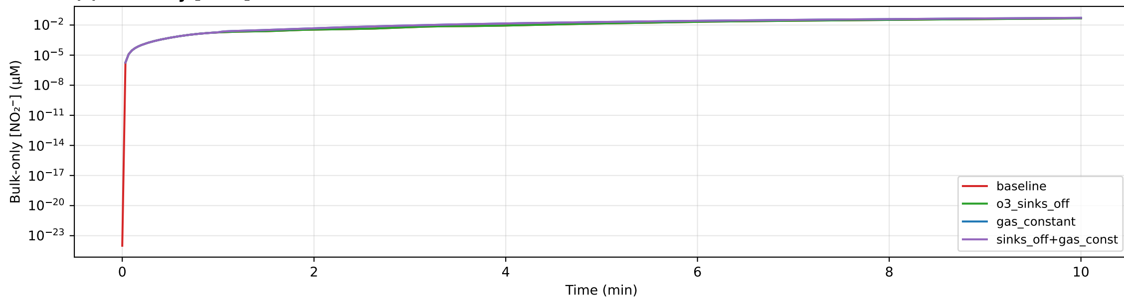
(c) Bulk-only [NO 2 - ]
