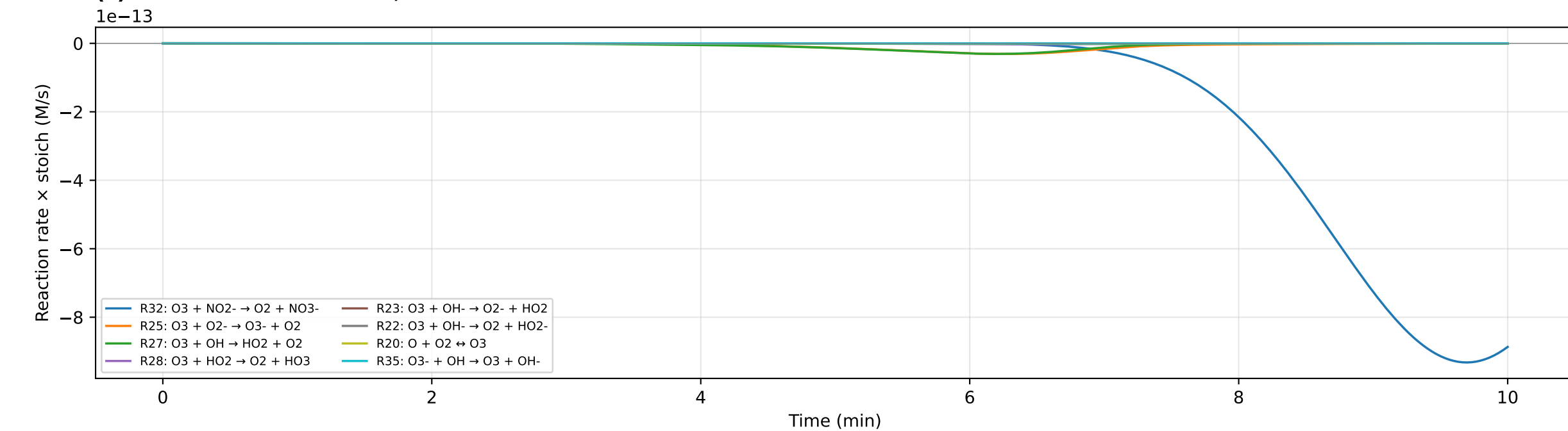
(c) Per-reaction O 3 source/sink at cell 40
