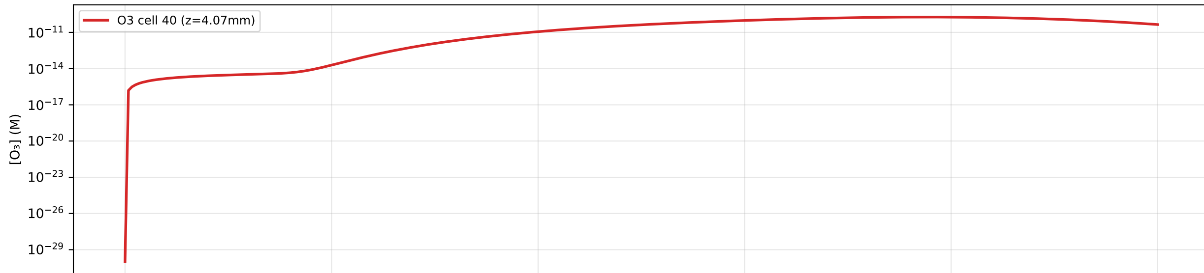
(a) [O 3 ] time series at z=4.07mm
