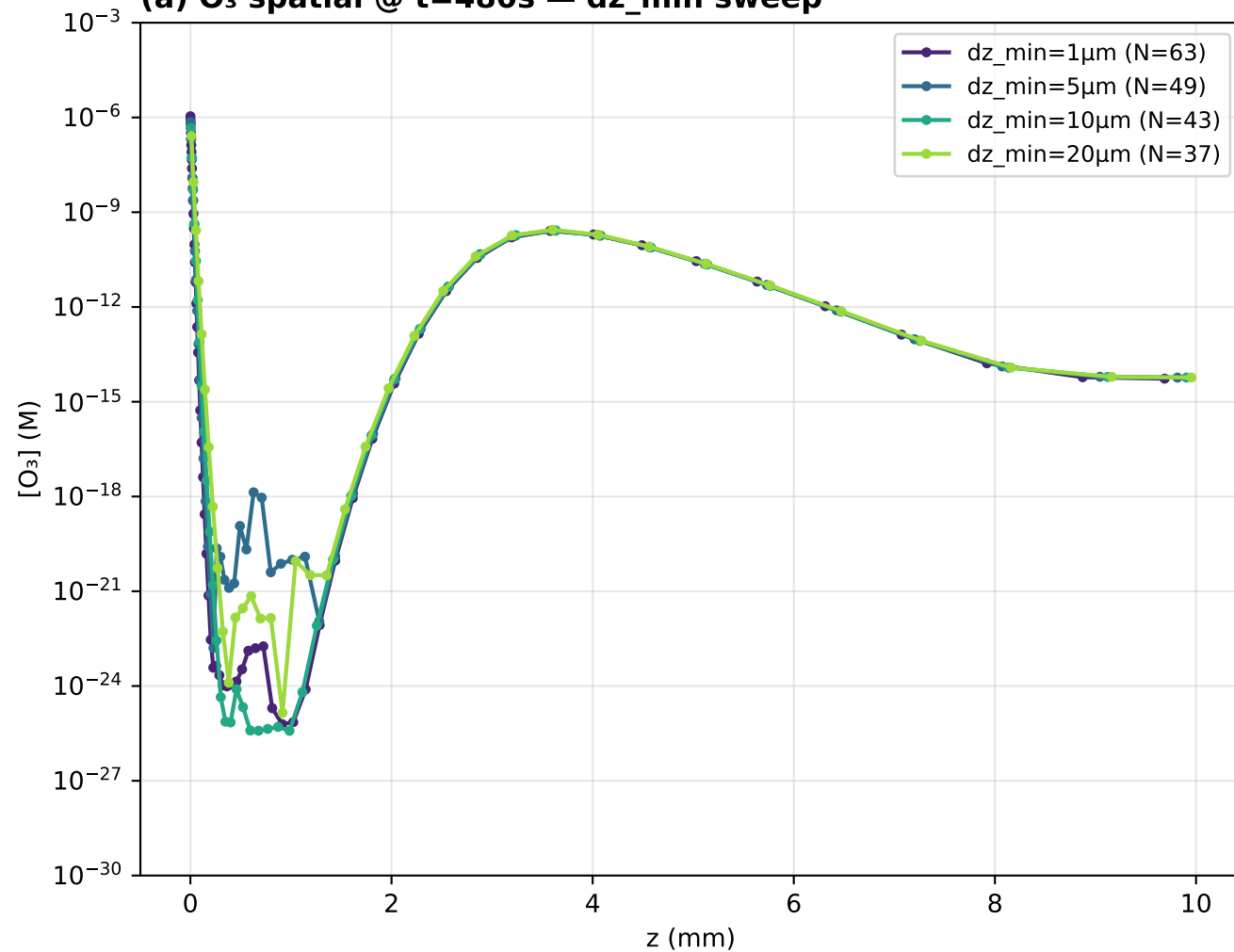
(a) O 3 spatial @ t=480s — dz_min sweep
