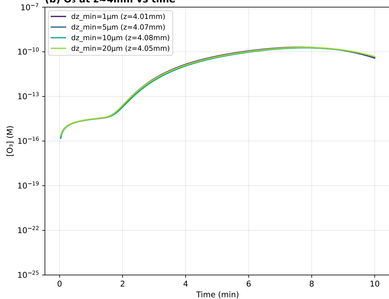
(b) O 3 at z≈4mm vs time
