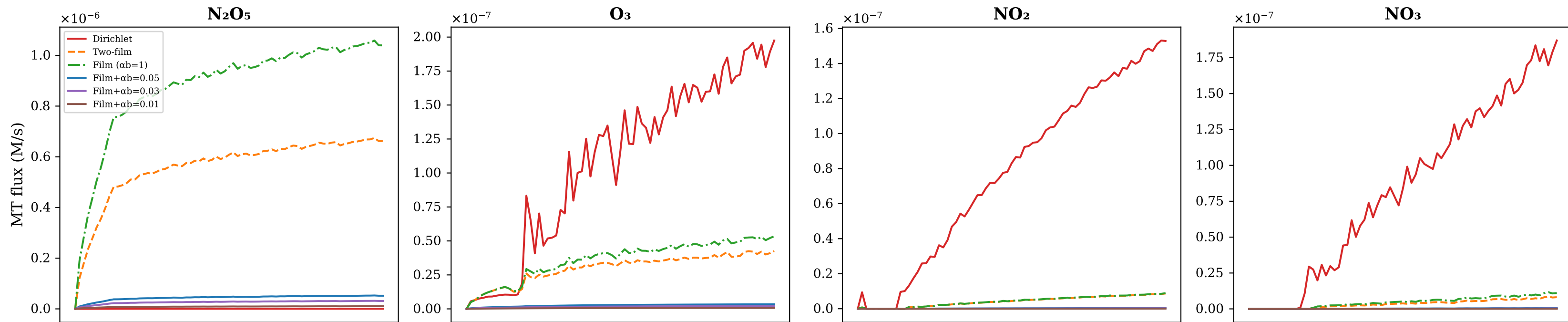
Mass transfer flux by BC model (DIW, 12 min)
