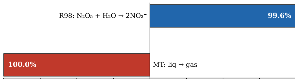
(a) \text{NO}_3^-
