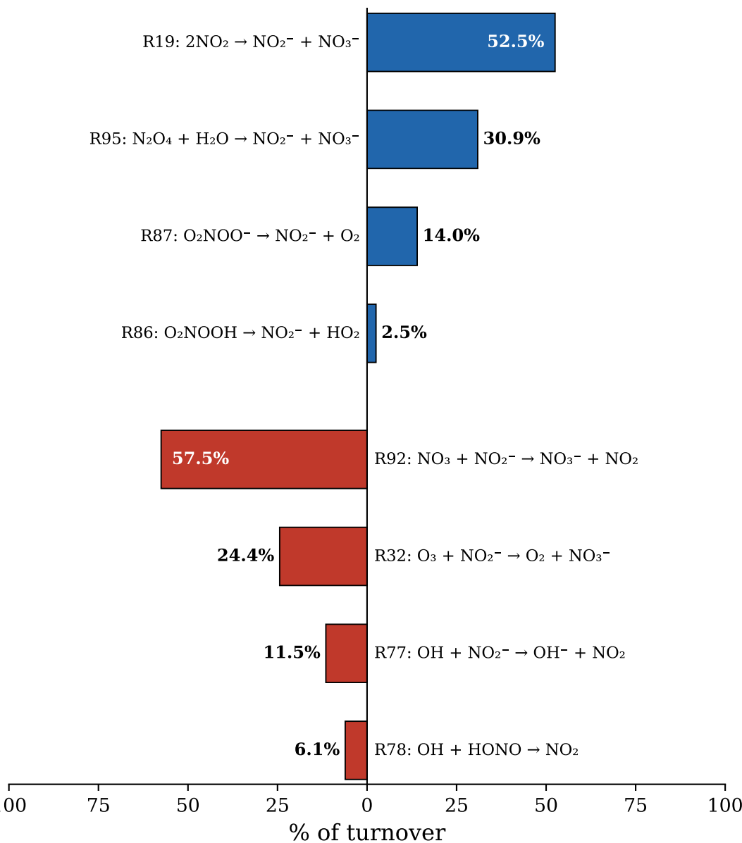
(c) \text{NO}_2^-
