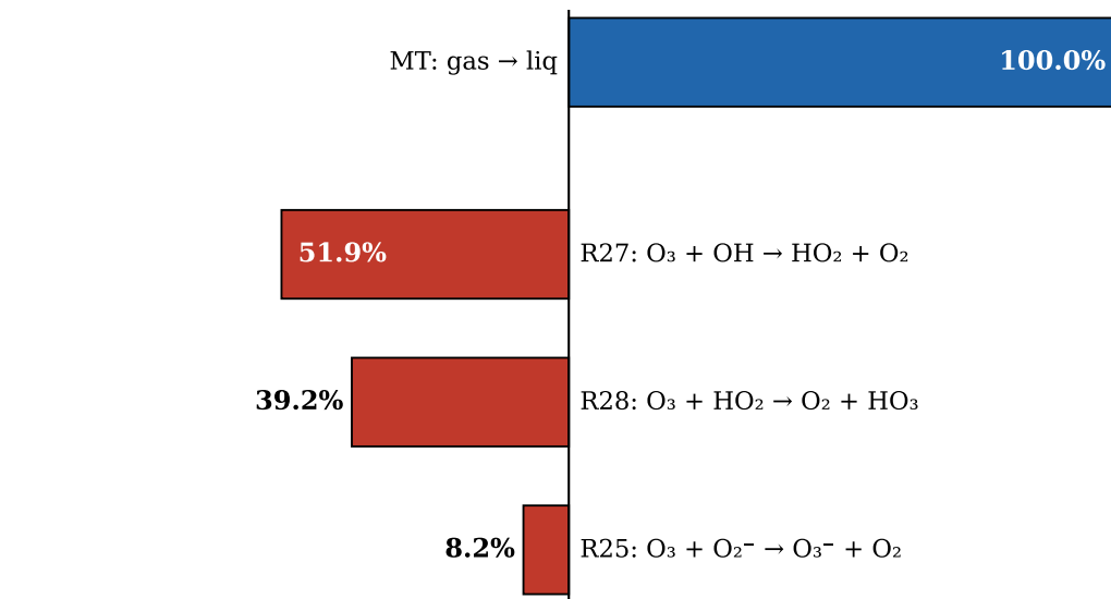
(b) \text{O}_3
