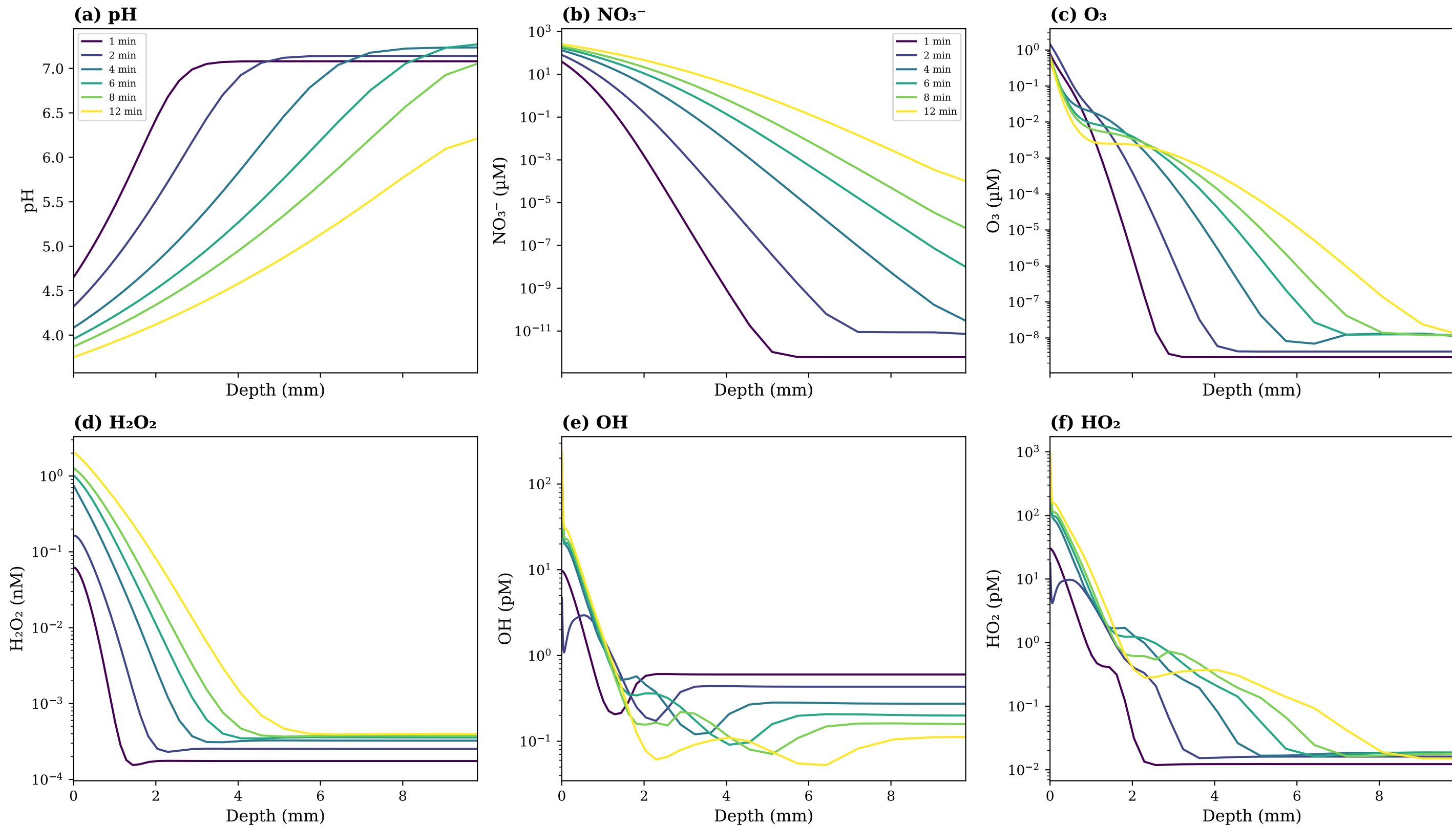
Spatial concentration profiles (DIW, Film+ \alpha b , \alpha b=0.03 )
