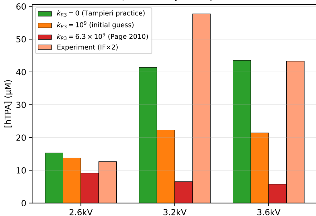
(a) k_{R3} sensitivity vs experiment
