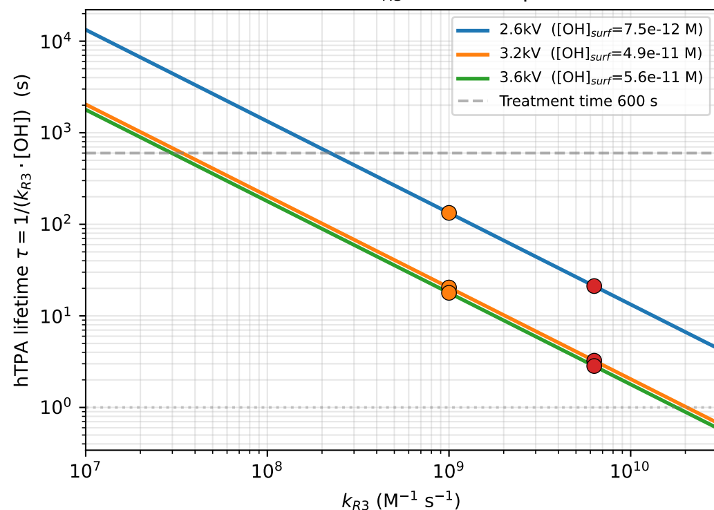
(b) hTPA lifetime: k_{R3} \times [\text{OH}] dependence
