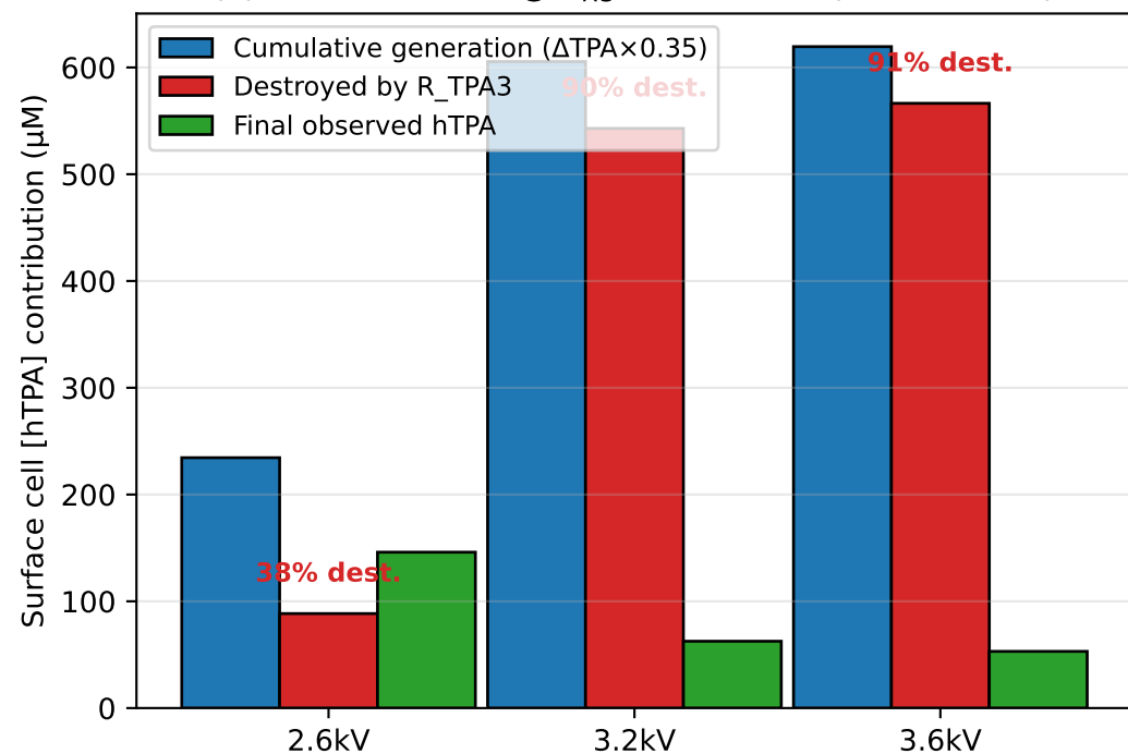
(c) Mass balance @ k_{R3} = 6.3 \times 10^9 (surface cell)
