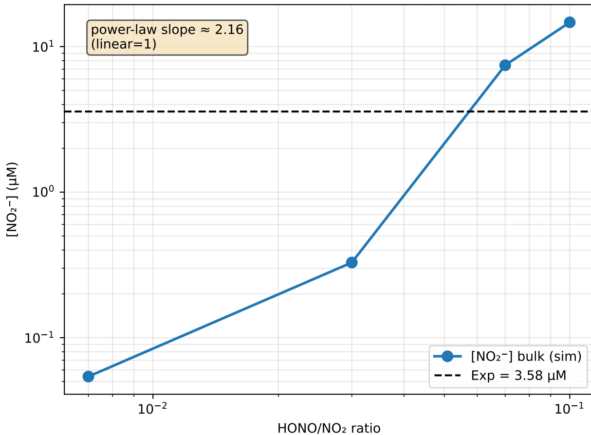
[NO 2 - ] bulk vs HONO ratio (log-log)
