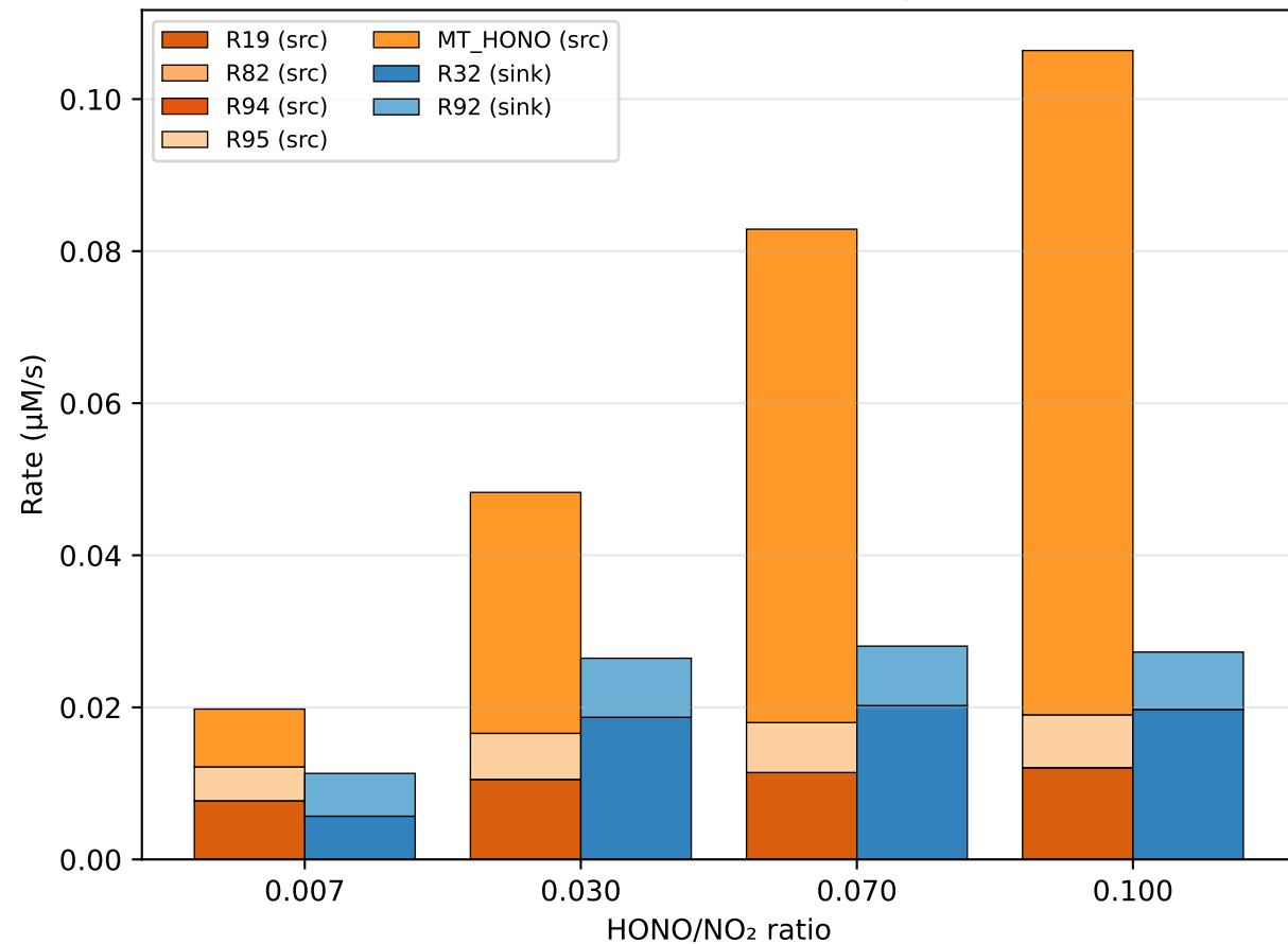
NO 2 - source & sink rates (bulk-avg at t=600s)
