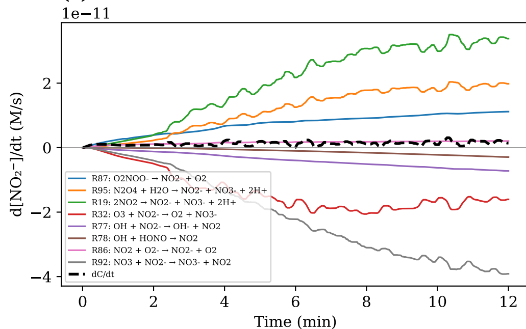
(c) NO 2 -
