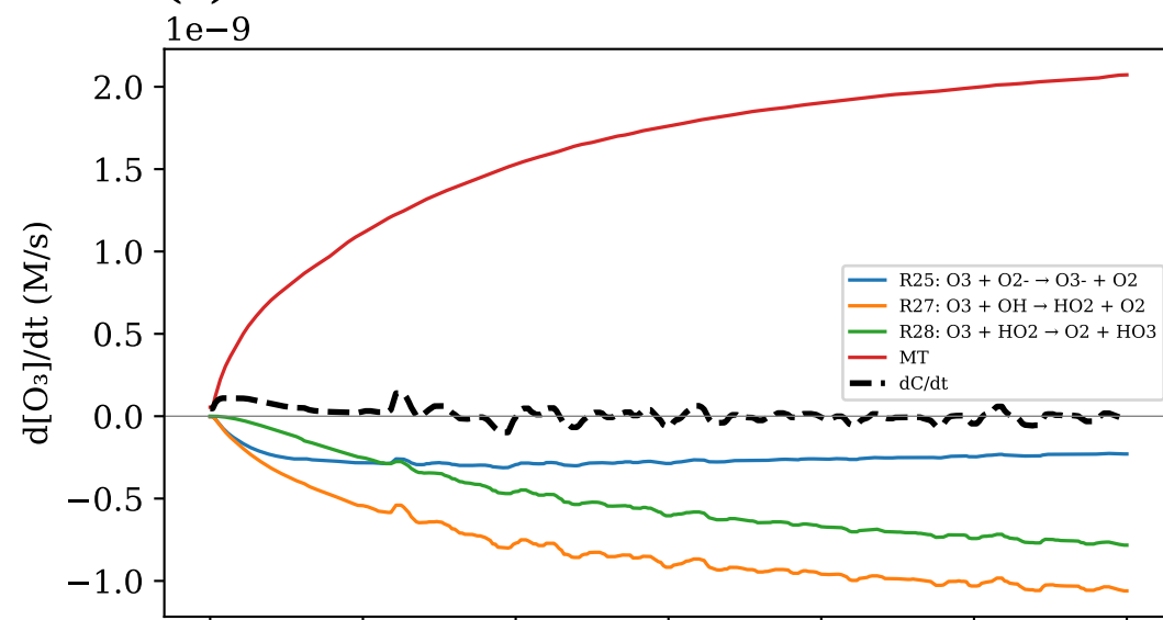
(b) O 3
