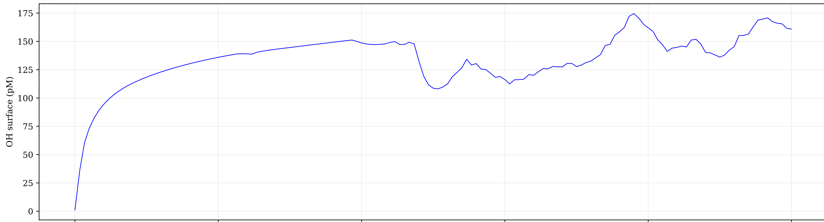
(b) OH surface: per-reaction rates
