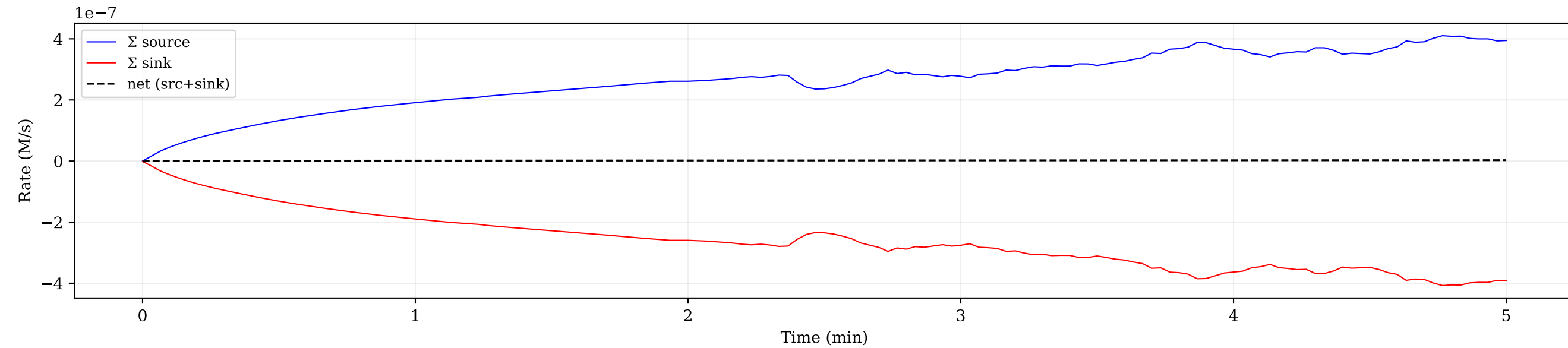
(c) OH surface: total source vs sink vs net
