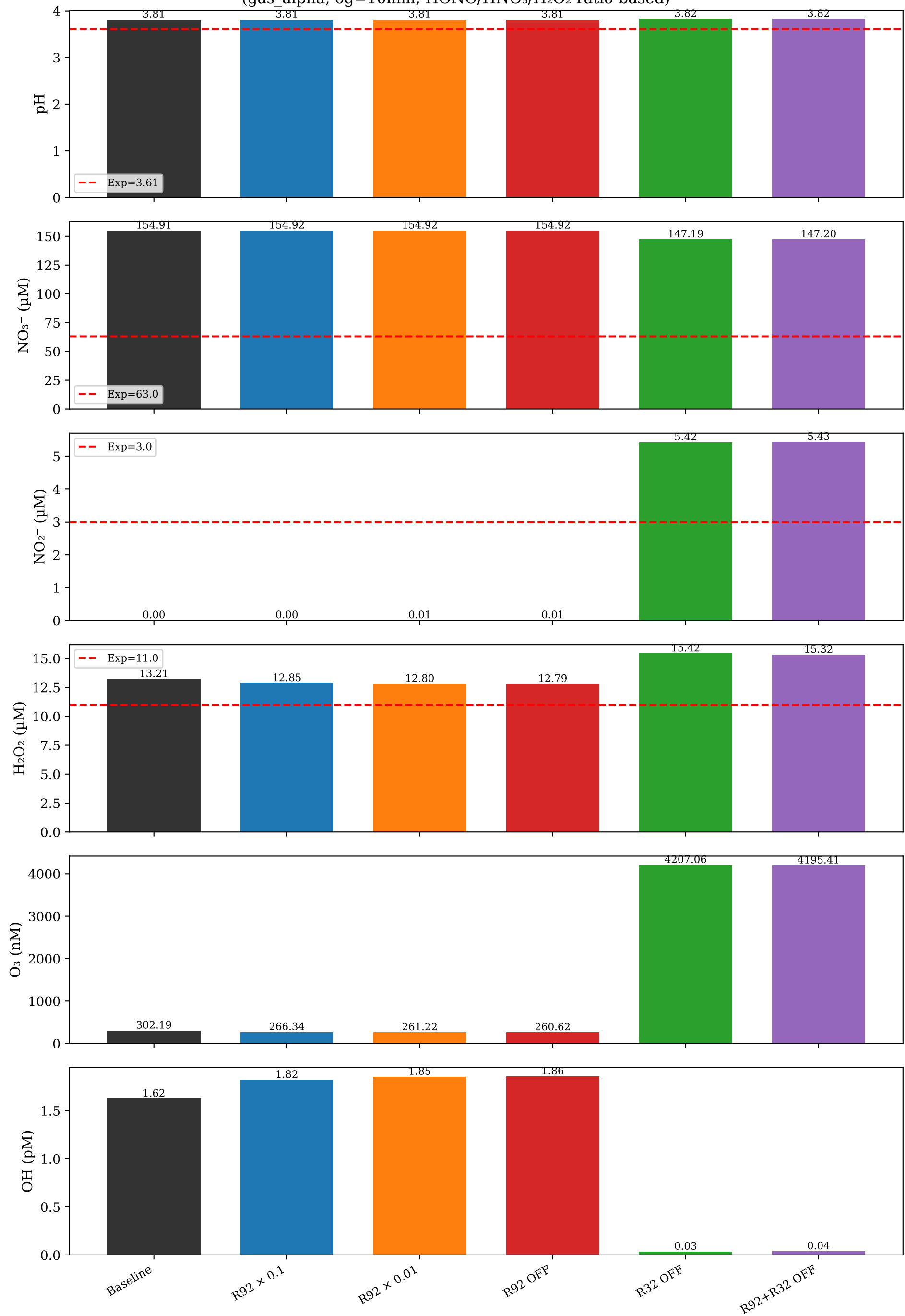
NO 2 - sensitivity: R92/R32 rate constant scaling (gas_alpha, δg=10mm, HONO/HNO 3 /H 2 O 2 ratio-based)
