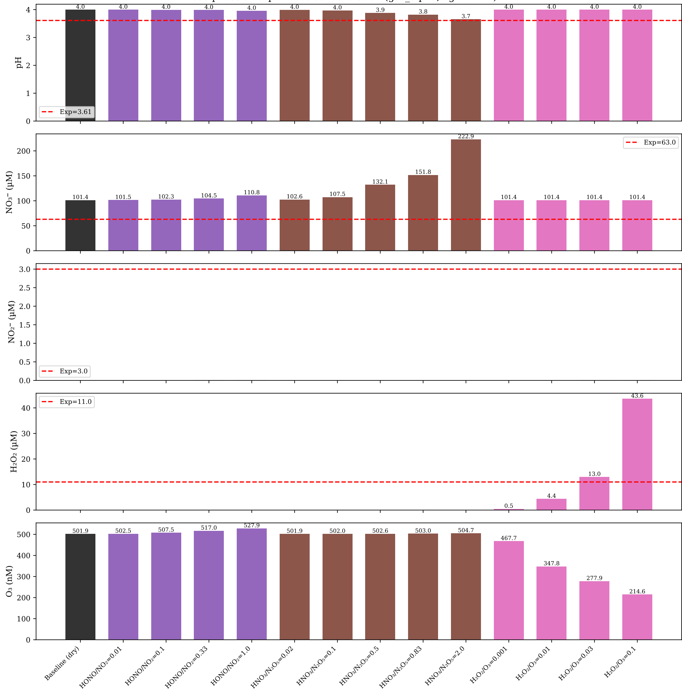
Gas-phase sweep: RONS concentration (gas_alpha, \delta g=10\text{mm} )
