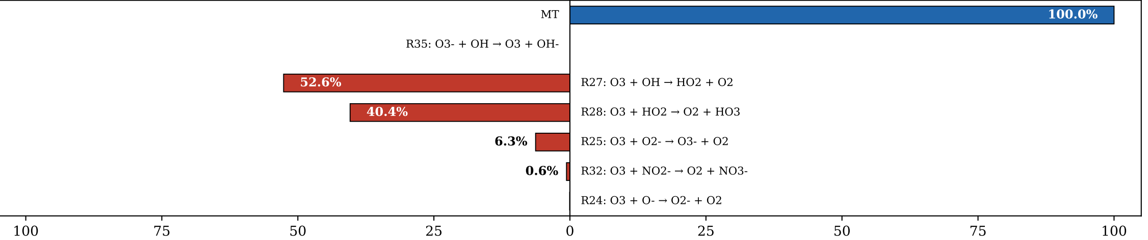
(c) \text{NO}_2^- ( \Sigma_{\text{src}} = 6.14\text{e-}11 \text{ M/s} )
