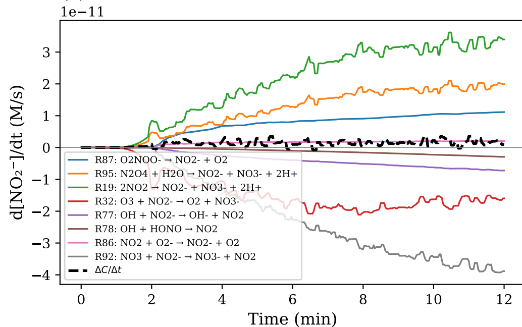
(c) \text{NO}_2^-
