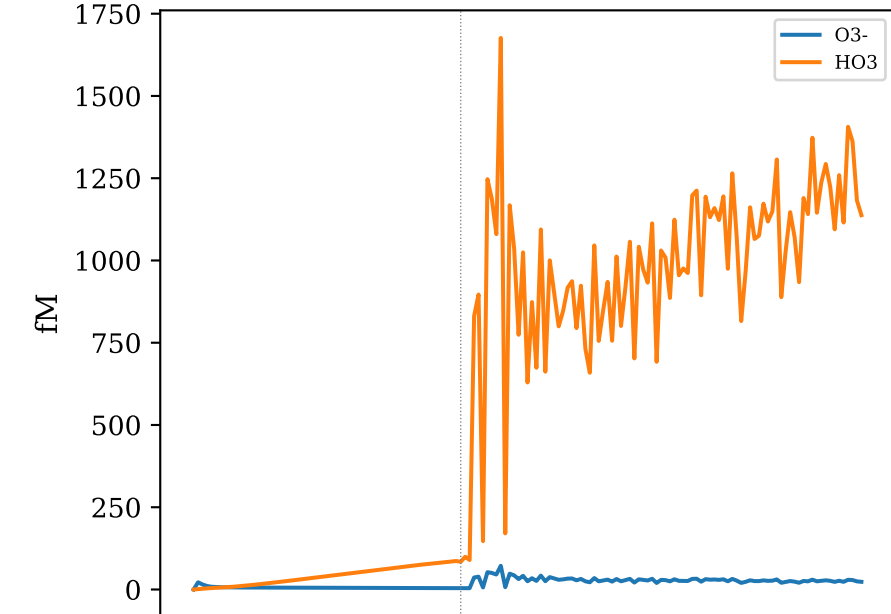
(c) O 3 - vs HO 3 (surface)
