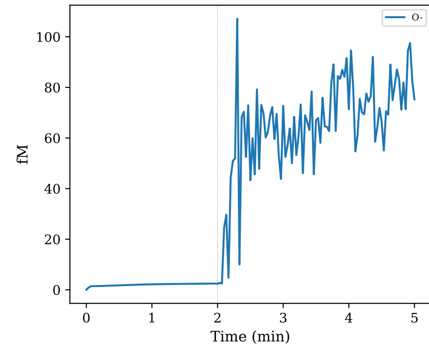
(f) O - (surface)
