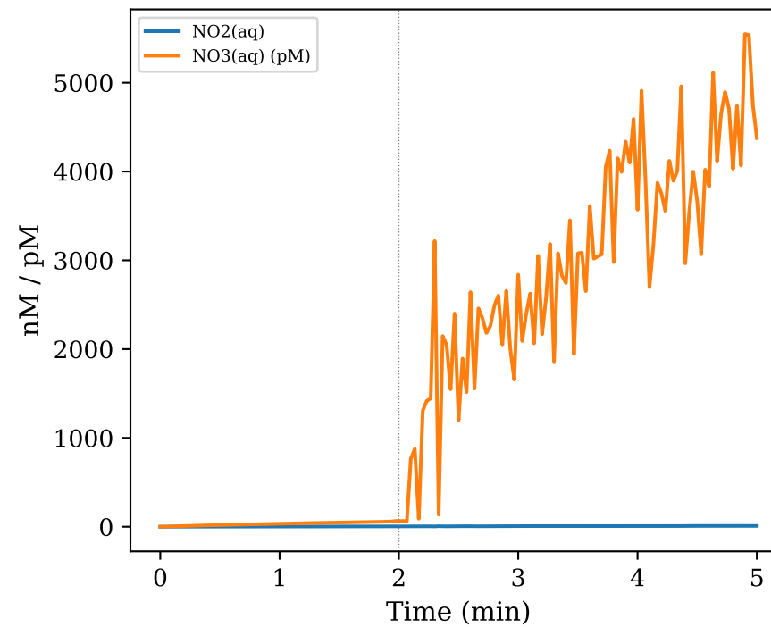
(e) dissolved NO 2 & NO 3 (surface)
