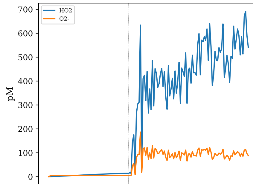
(b) HO 2 vs O 2 - (surface)
