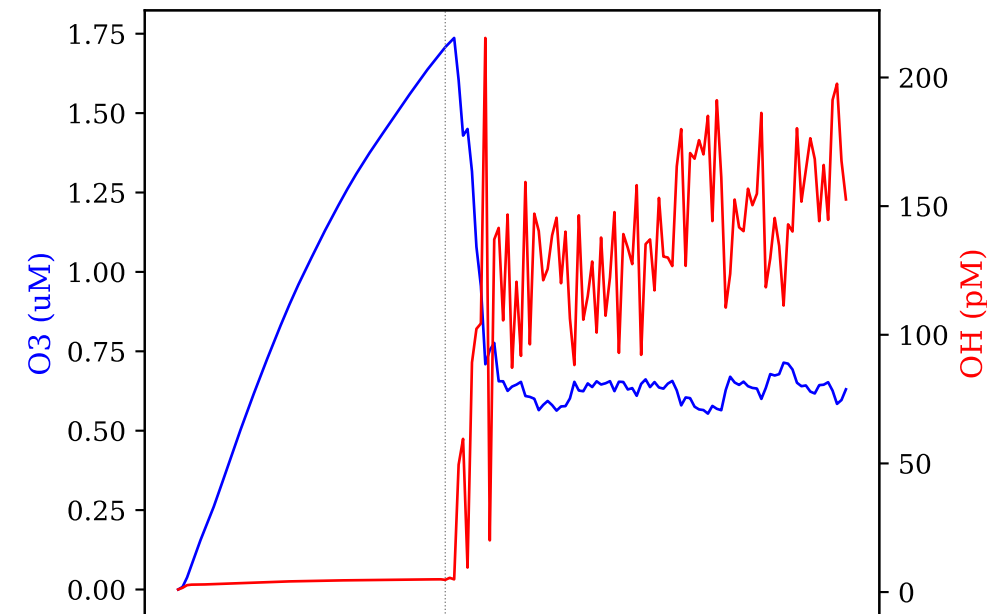
(a) O 3 vs OH (surface)
