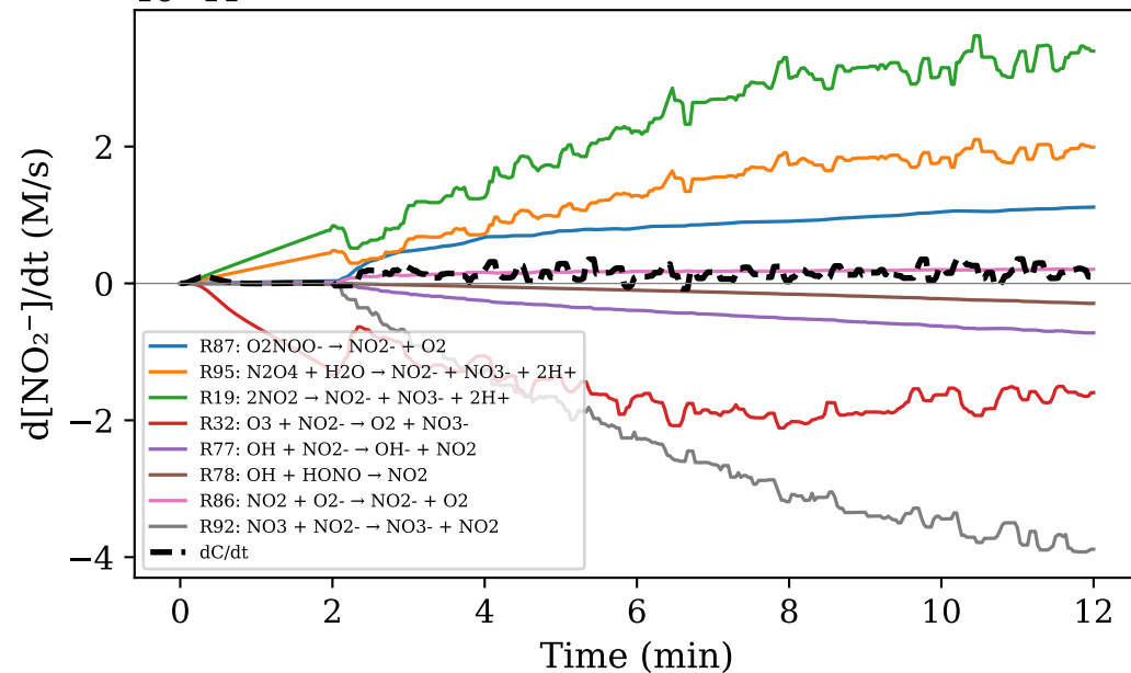
(c) \text{NO}_2^-
