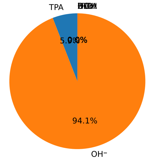
(f) OH sinks @ 3.2kV, t=600s (total rate = 1.67 \times 10^{-5} M/s)
