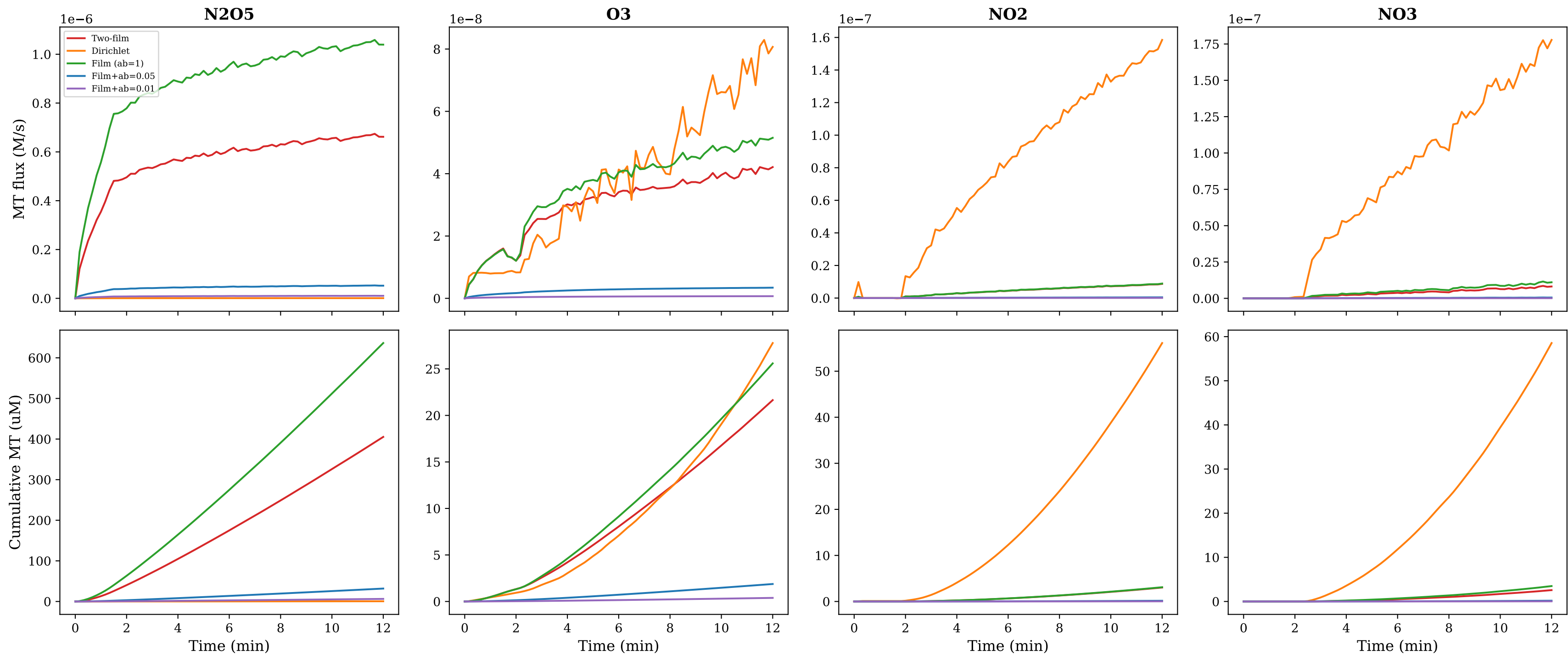
Mass transfer flux by BC model (DIW, 12 min)
