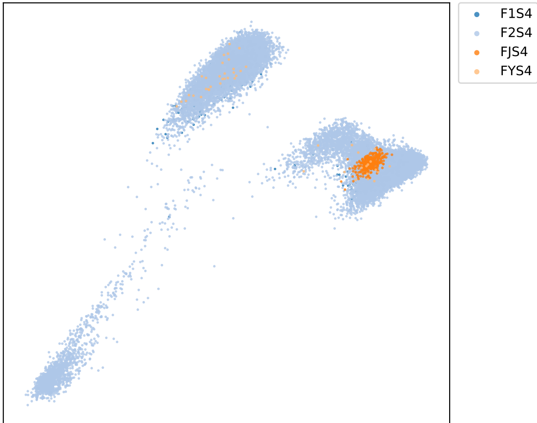
PCA colored by sample_prefix1
