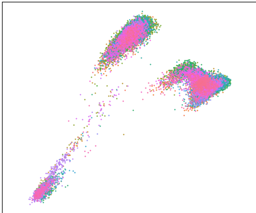
PCA colored by sample_prefix2
