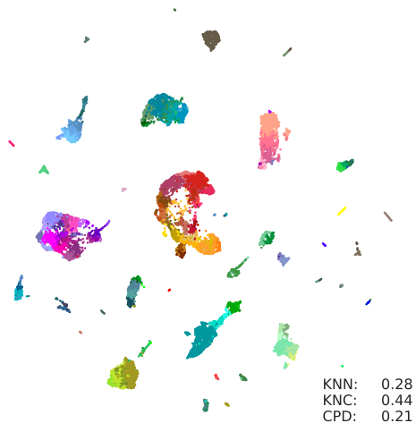
Latent: SCVI_N20 Tasic et al. 2018 min_dist=0.1, n_neighbors=15
