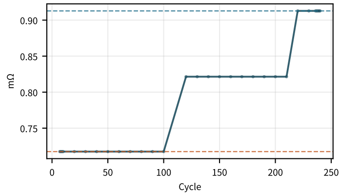
R _{ct} (SOC50) increasing · +0.0883/100
