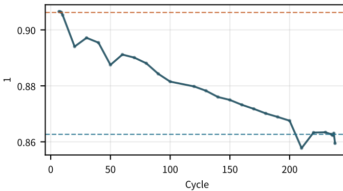
전압 효율 flat · -0.0183/100
