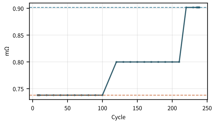
R _{ct} (SOC50) increasing · +0.0697/100
