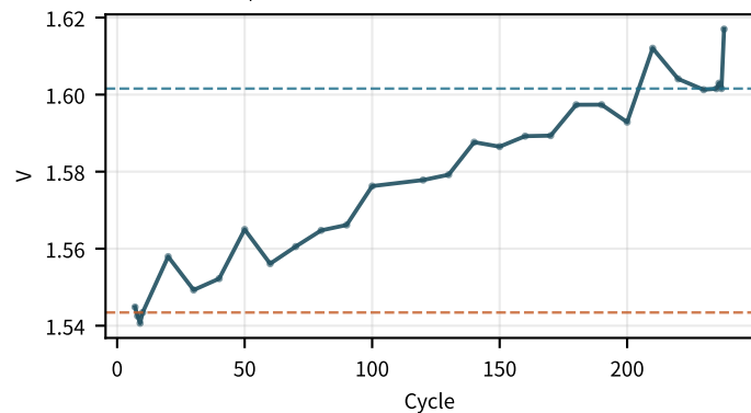
max dV 고SOC flat · +0.0274/100
