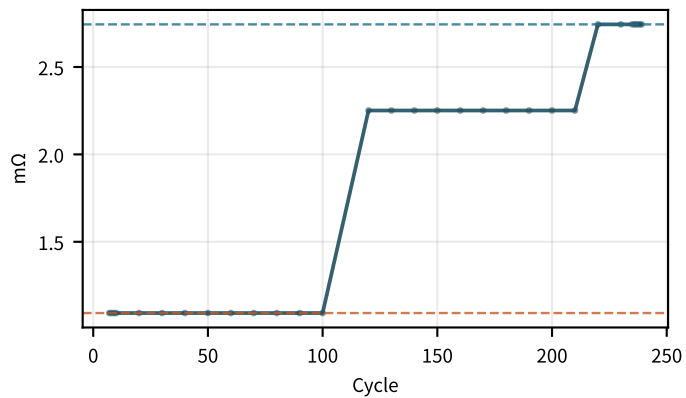
R \Omega (SOC50) increasing · +0.798/100
