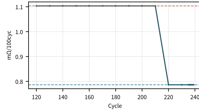
RΩ 성장률 /100cyc decreasing · -0.321/100
