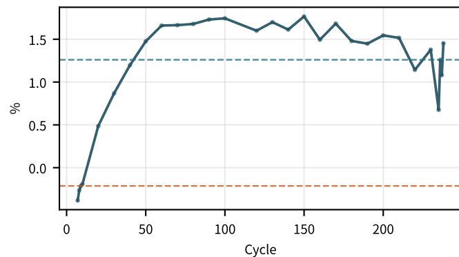
LLI 곡선 proxy increasing · +0.402/100
