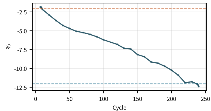
LAM 곡선 proxy decreasing · -4.23/100
