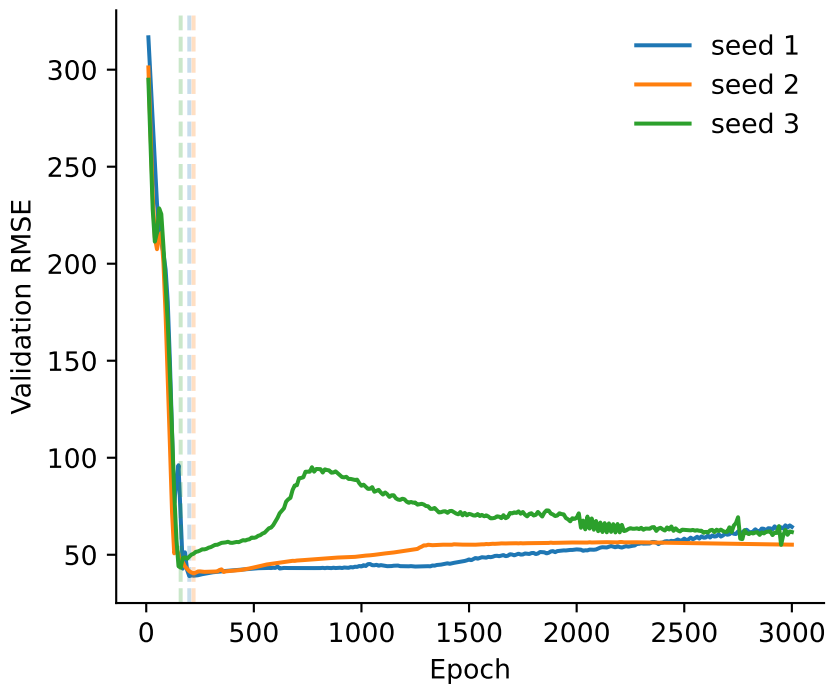
LSTM-NN
