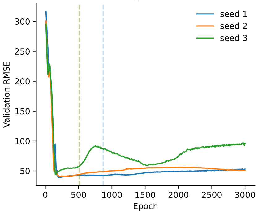
Logi-PINN
