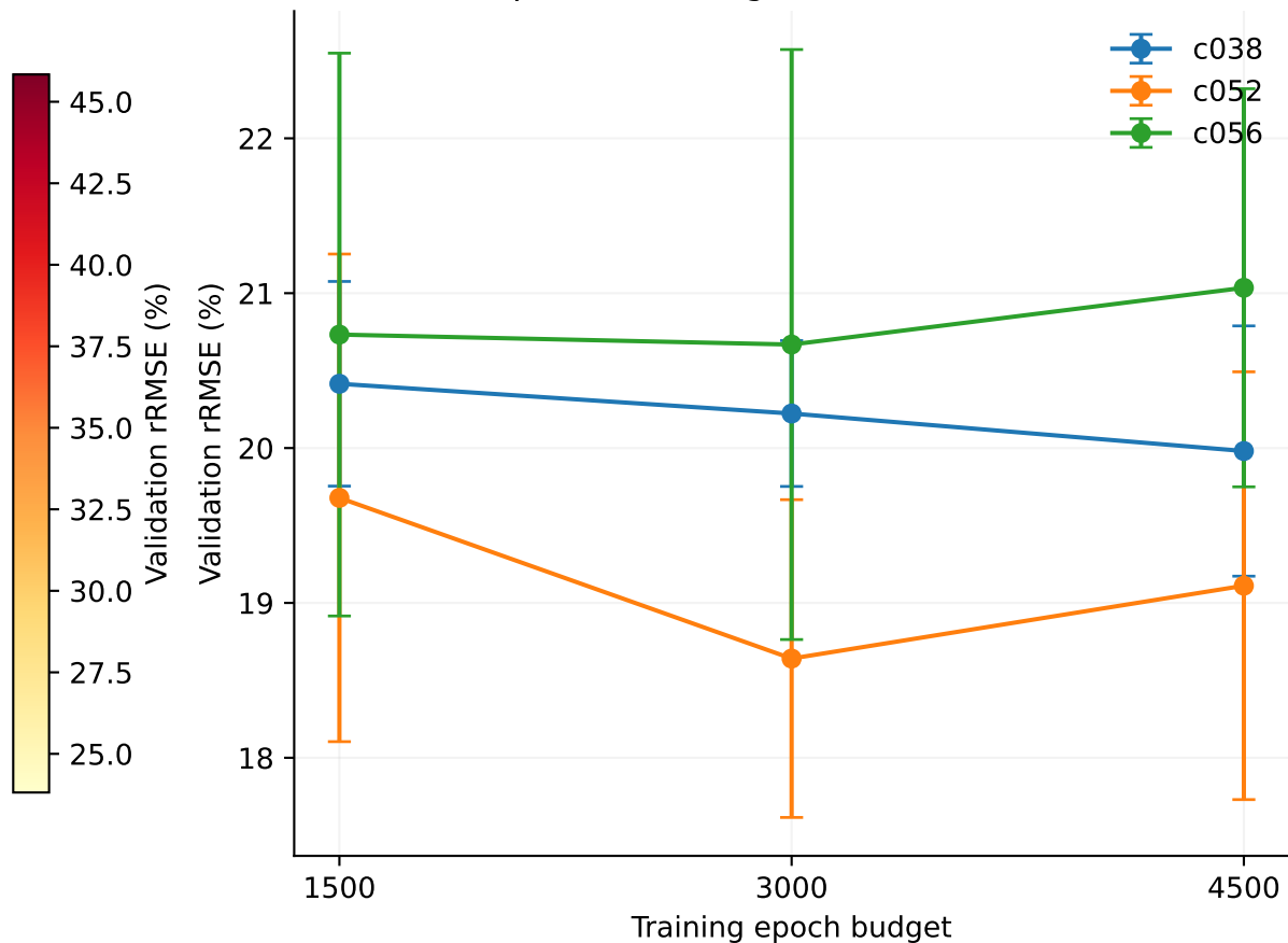
Top three settings · mean \pm seed SD
