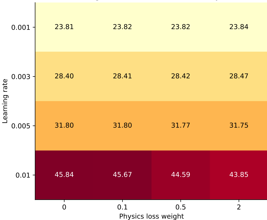
Original architecture · seed 1 only
