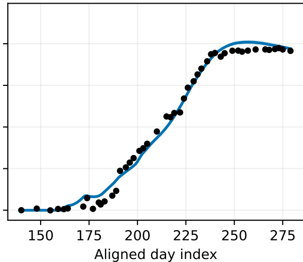
Genotype 133
