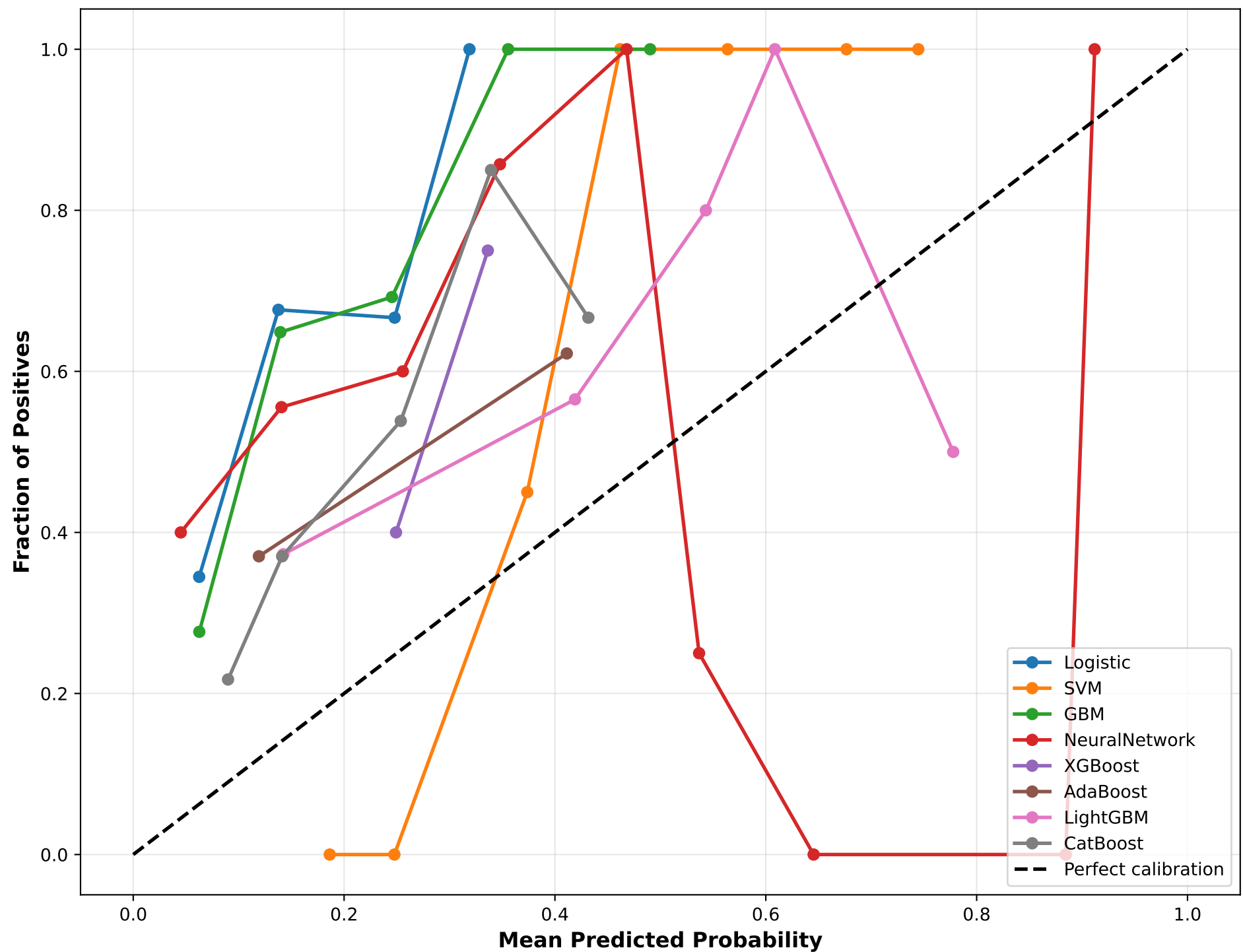
Calibration Curve - External Set
