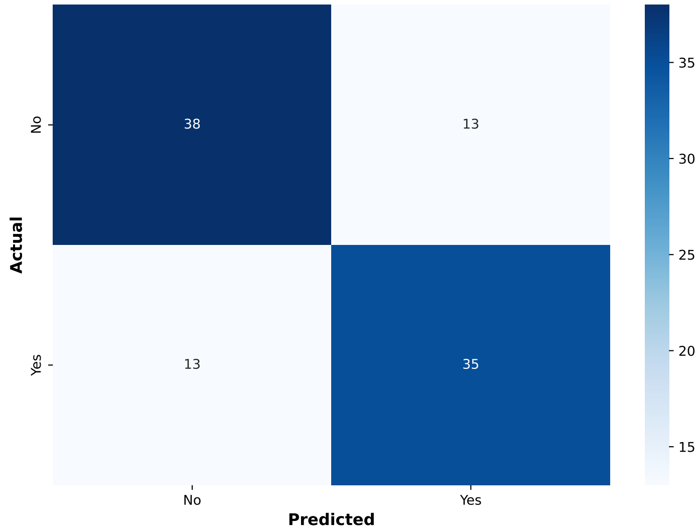
GBM - External Set
