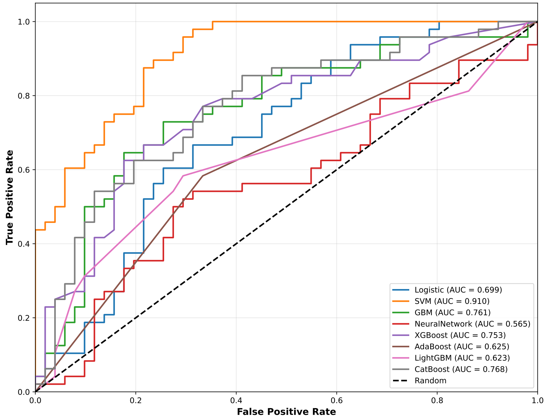
ROC Curve - External Set
