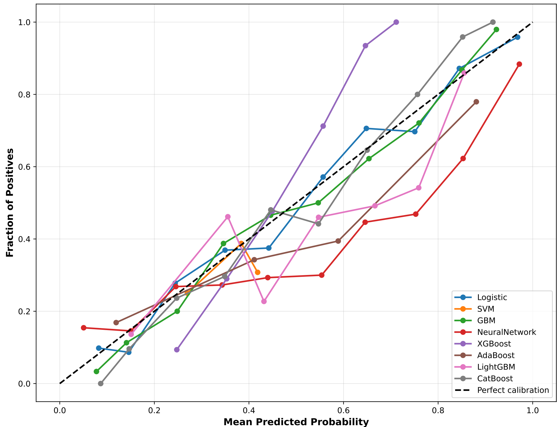
Calibration Curve - Test Set
